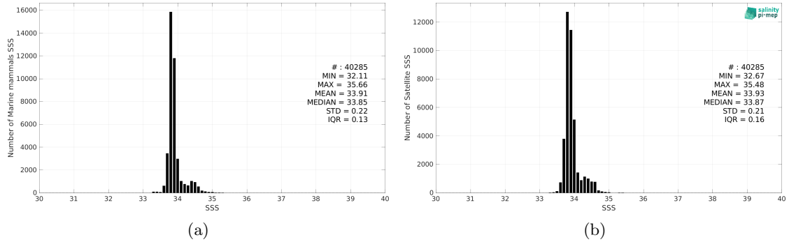
Figure 2: Histograms of SSS from Marine mammals (a) and Aquarius SSS L4 OI v5 - Monthly (IPRC) (b) considering all match-up pairs per bins of 0.1 over the Roaring Forties and Furious Fifties Pi-MEP region and for the full satellite product period.
