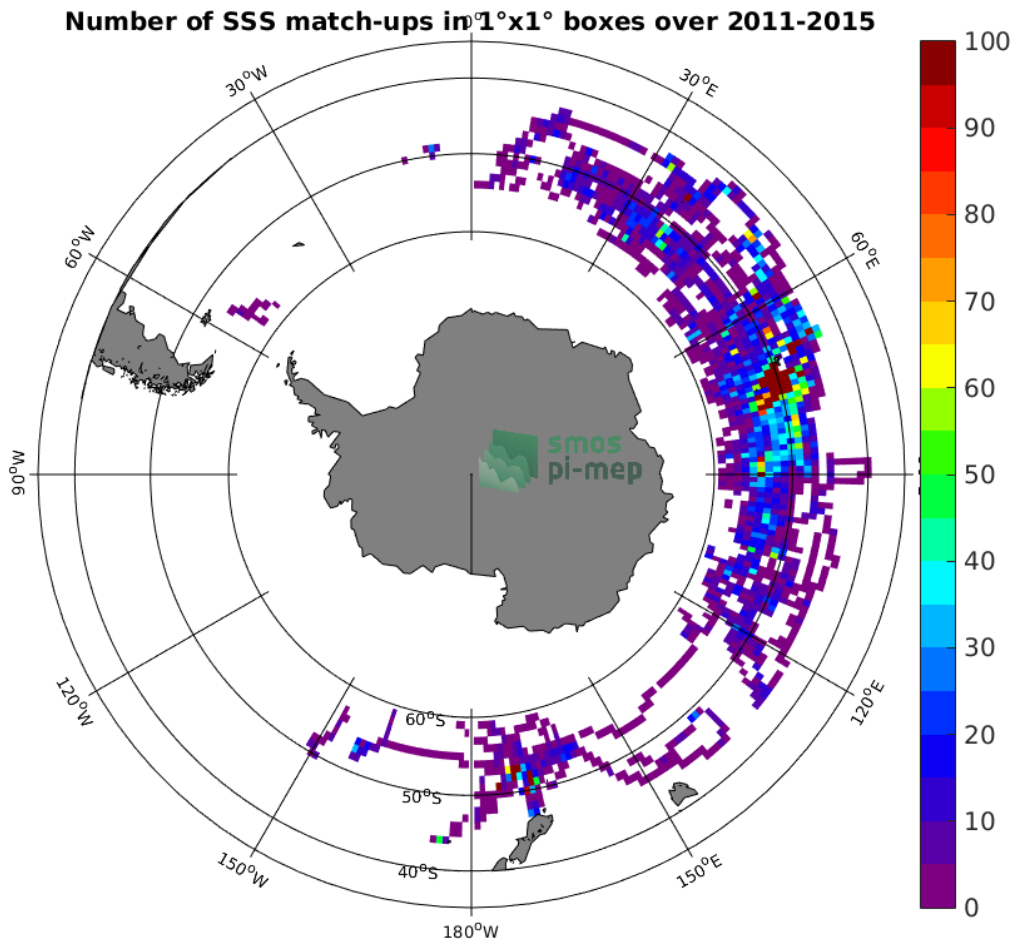
Figure 4: Number of SSS match-ups between Sea mammals SSS and the Aquarius-L4-IPRC-V5-MONTHLY SSS product for the Roaring Forties and Furious Fifties Pi-MEP region over 1°x1° boxes and for the full satellite product period.
