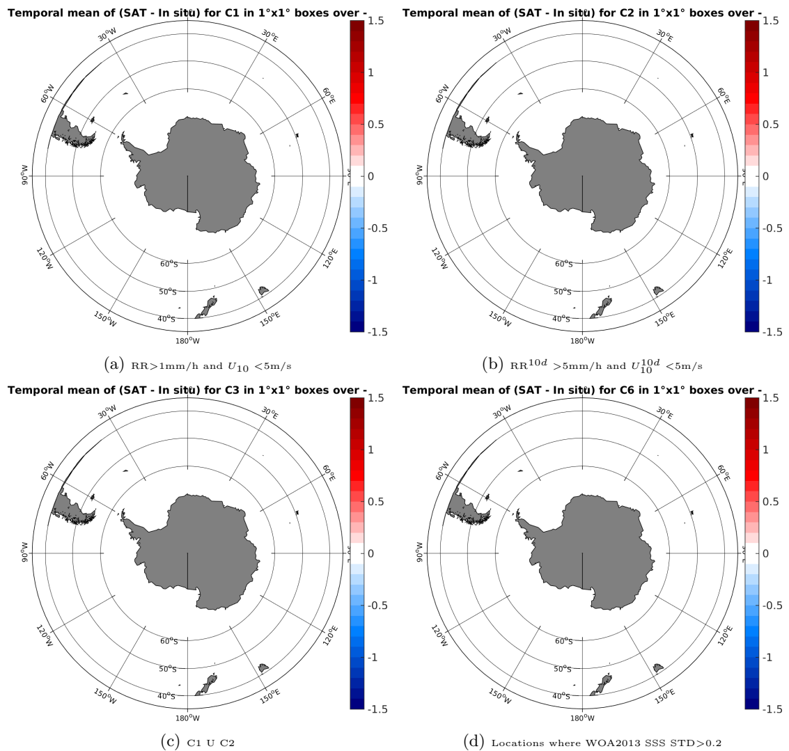
Figure 11: Temporal mean gridded over spatial boxes of size 1^\circ \times 1^\circ of \Delta SSS (Aquarius-L4-IPRC-V4-WEEKLY - Surface drifters) for 4 different subdatasets corresponding to:RR > 1 mm/h and U_{10} < 5 m/s (a), RR ^{10d} > 5 mm/h and U_{10}^{10d} < 5 m/s (b), C1 U C2 (c),Locations where WOA2013 SSS STD > 0.2 (d).
