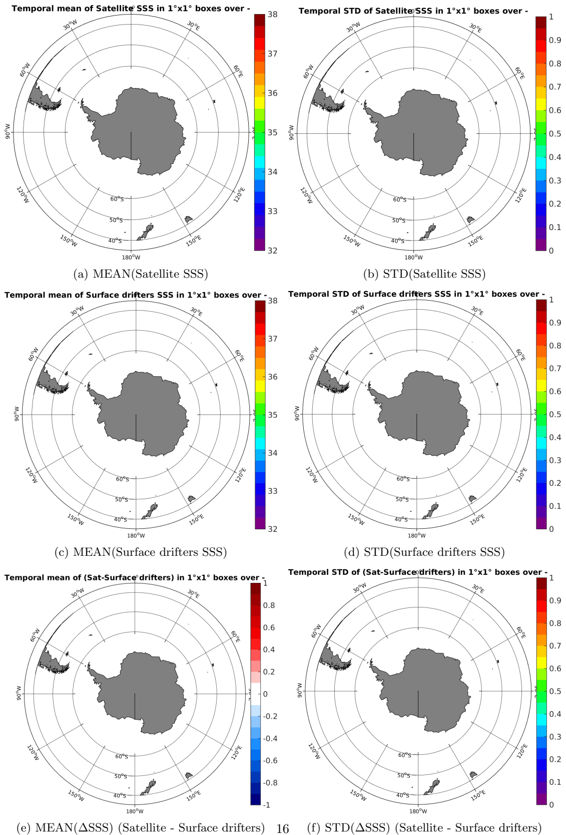
Figure 5: Temporal mean (left) and STD (right) of SSS from Aquarius-L4-IPRC-V4-WEEKLY (top), Surface drifters (middle), and of \Delta SSS (Satellite - Surface drifters). Only match-up pairs are used to generate these maps.
