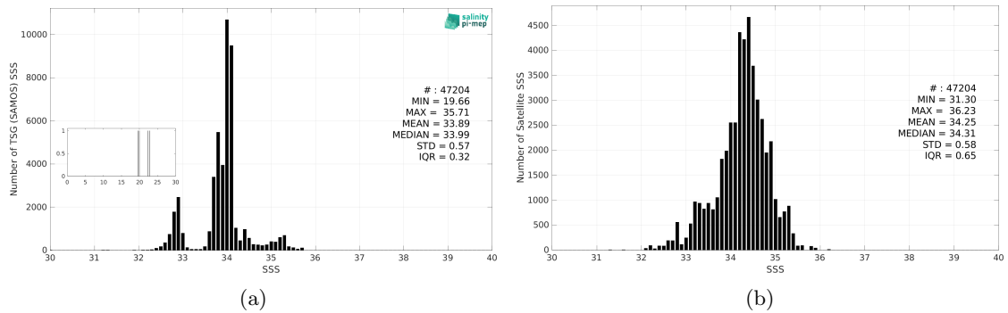
Figure 3: Histograms of SSS from TSG (SAMOS) (a) and Aquarius SSS L3 CAP v5 - 7-Day running (JPL) (b) considering all match-up pairs per bins of 0.1 over the Roaring Forties and Furious Fifties Pi-MEP region and for the full satellite product period.
