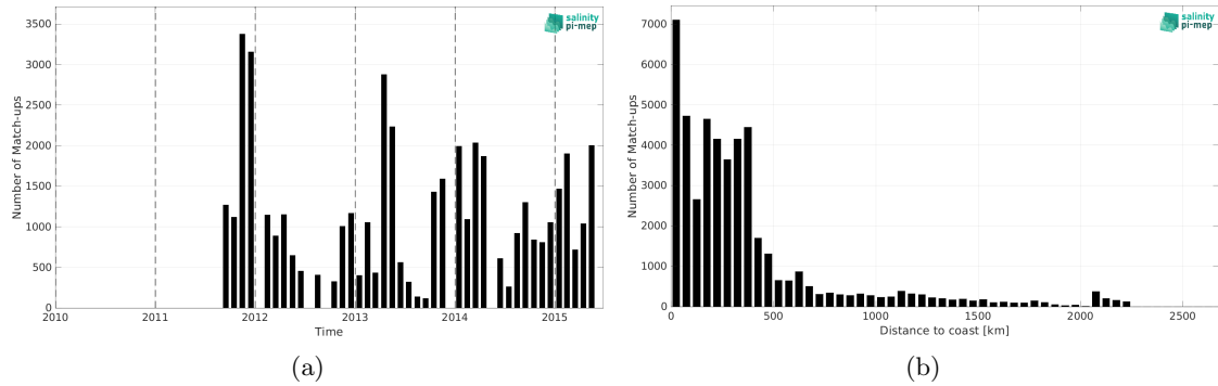
Figure 2: Number of match-ups between TSG (SAMOS) and Aquarius SSS L3 CAP v5 - 7-Day running (JPL) SSS as a function of time (a) and as function of the distance to coast (b) over the Roaring Forties and Furious Fifties Pi-MEP region and for the full satellite product period.
