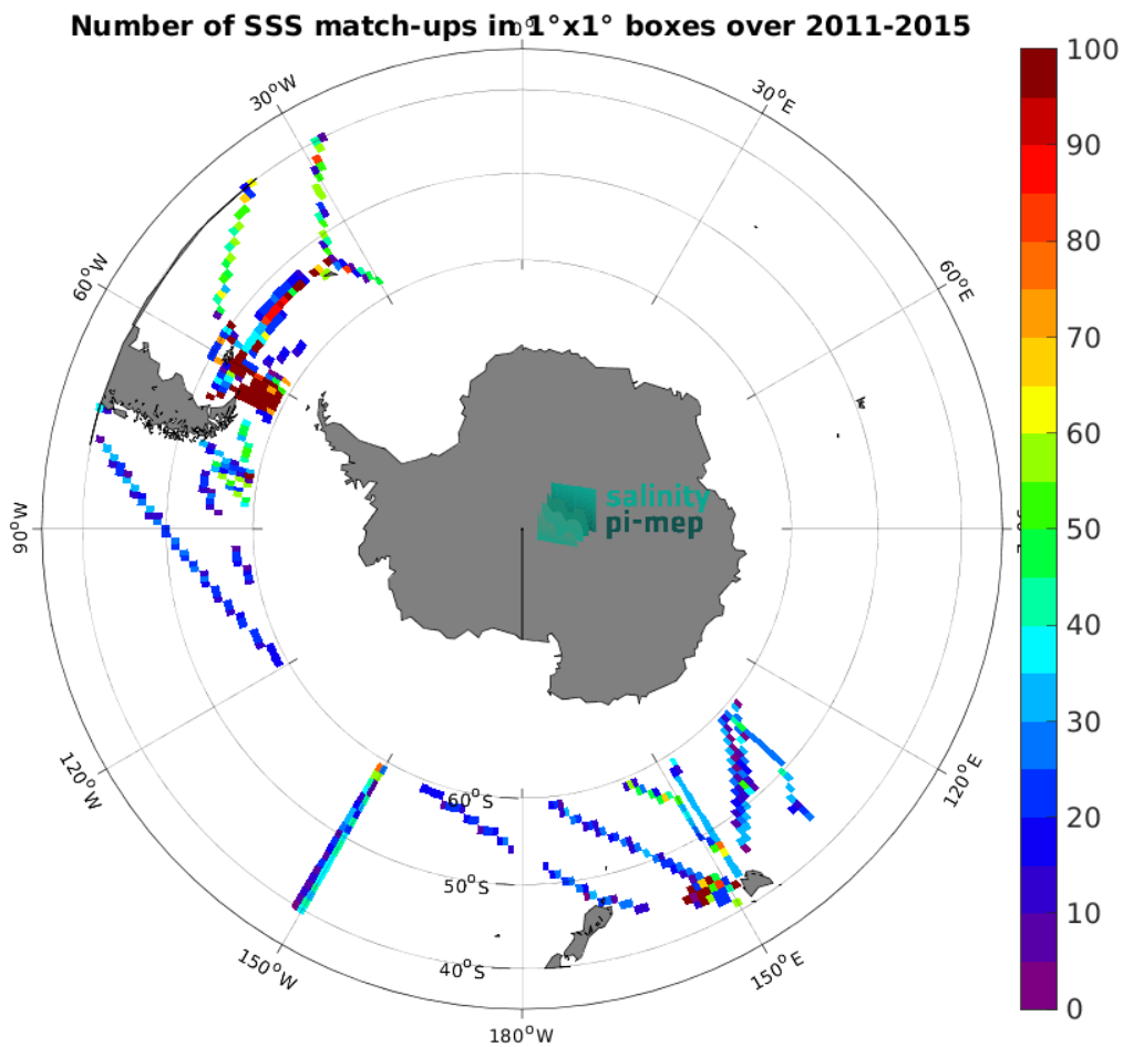
Figure 5: Number of SSS match-ups between TSG (SAMOS) SSS and the Aquarius SSS L3 CAP v5 - 7-Day running (JPL) SSS product for the Roaring Forties and Furious Fifties Pi-MEP region over 1^\circ \times 1^\circ boxes and for the full satellite product period.
