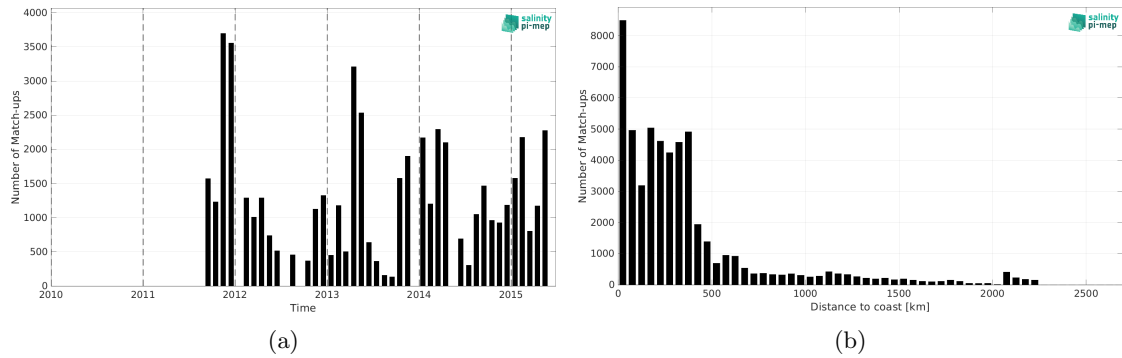
Figure 1: Number of match-ups between TSG (SAMOS) and Aquarius SSS L3 CAP v5 - 7-Day running (JPL) SSS as a function of time (a) and as function of the distance to coast (b) over the Roaring Forties and Furious Fifties Pi-MEP region and for the full satellite product period.
