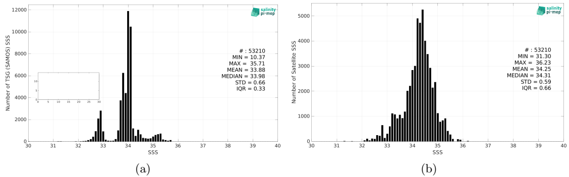
Figure 2: Histograms of SSS from TSG (SAMOS) (a) and Aquarius SSS L3 CAP v5 - 7-Day running (JPL) (b) considering all match-up pairs per bins of 0.1 over the Roaring Forties and Furious Fifties Pi-MEP region and for the full satellite product period.
