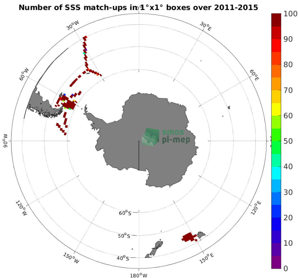
Figure 4: Number of SSS match-ups between TSG (SAMOS) SSS and the Aquarius SSS L3 CAP v5 - 7-Day running (JPL) SSS product for the Roaring Forties and Furious Fifties Pi-MEP region over 1^\circ \times 1^\circ boxes and for the full satellite product period.
