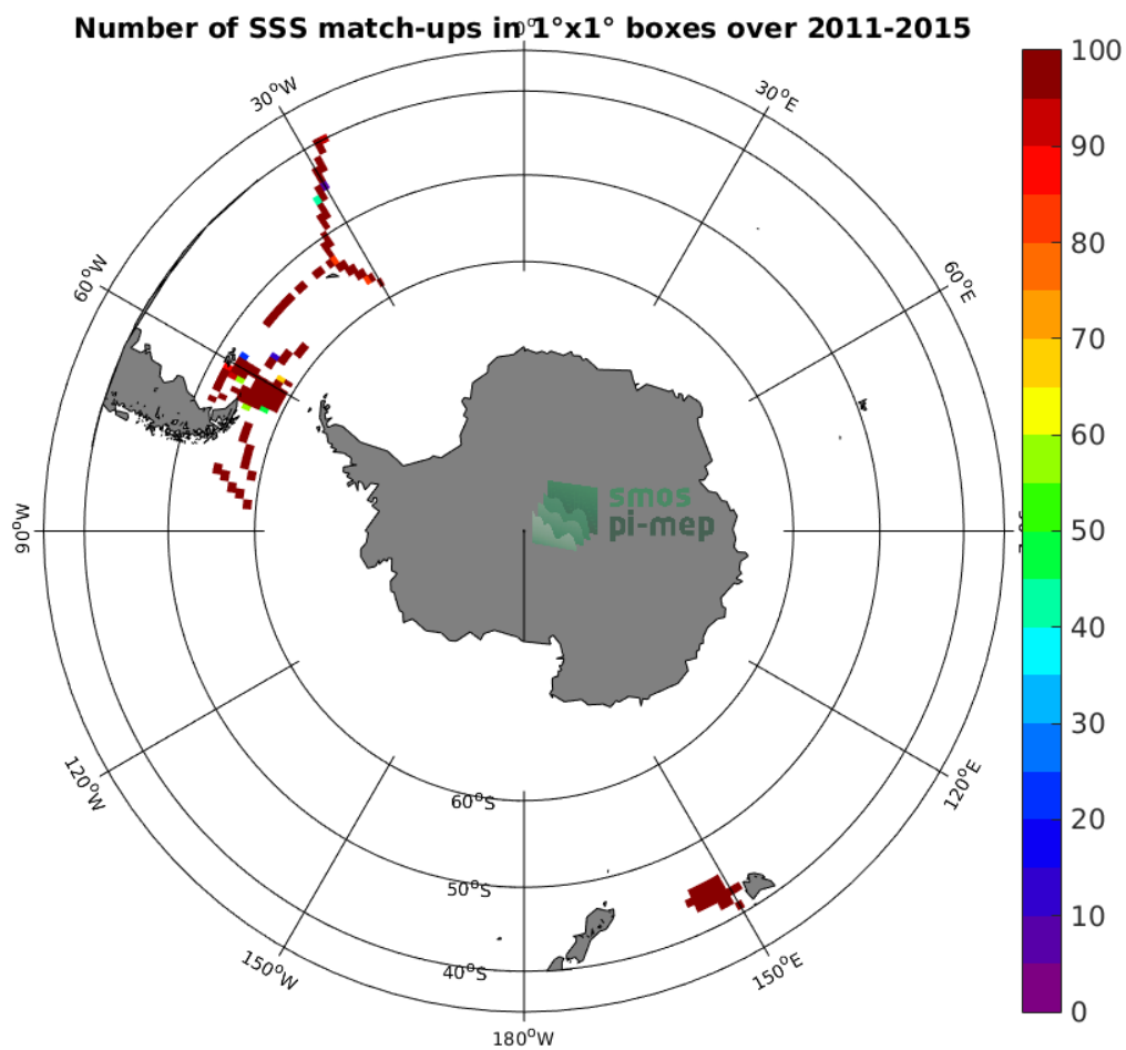
Figure 4: Number of SSS match-ups between TSG-SAMOS SSS and the Aquarius-L3-JPL-V5-7DAY-RUNNING SSS product for the Roaring Forties and Furious Fifties Pi-MEP region over 1^{\circ} \times 1^{\circ} boxes and for the full satellite product period.
