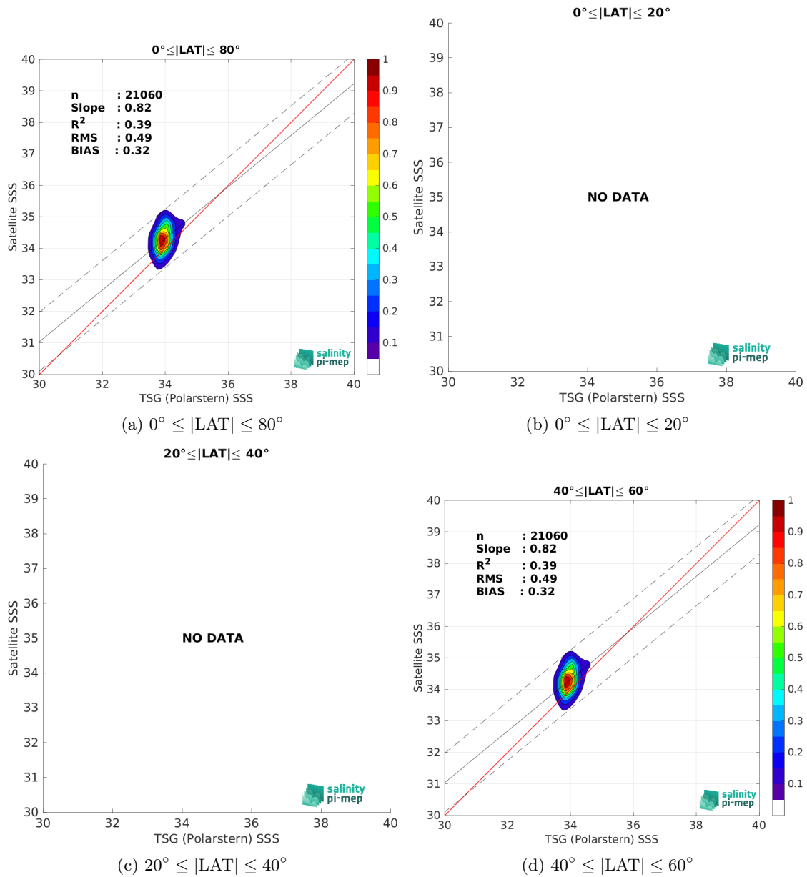
Figure 10: Contour maps of the concentration of Aquarius SSS L3 CAP v5 - 7-Day running (JPL) SSS (y-axis) versus TSG (Polarstern) SSS (x-axis) at match-up pairs for different latitude bands. For each plot, the red line shows x=y . The black thin and dashed lines indicate a linear fit through the data cloud and the \pm 95\% confidence levels, respectively. The number match-up pairs n , the slope and R^2 coefficient of the linear fit, the root mean square (RMS) and the mean bias between satellite and in situ data are indicated for each latitude band in each plots.
