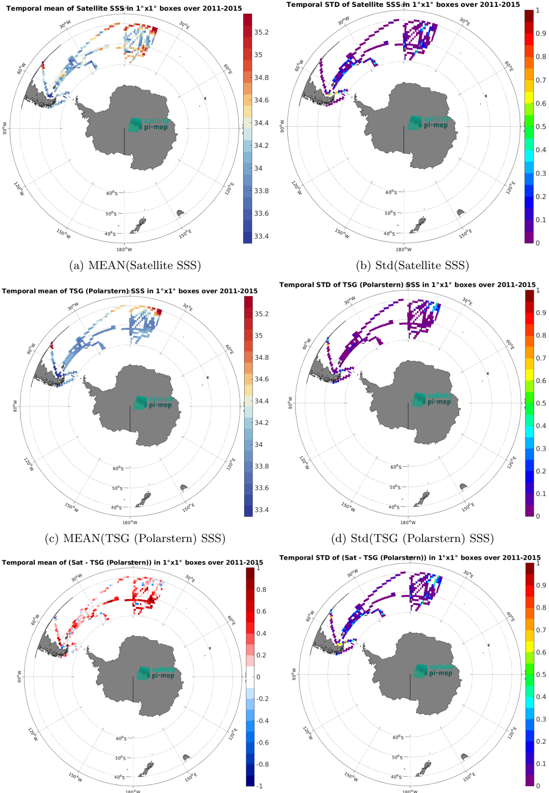
Figure 7: Temporal mean (left) and Std (right) of SSS from Aquarius SSS L3 CAP v5 - 7-Day running (JPL) (top), TSG (Polarstern) (middle), and of \Delta SSS (Satellite - TSG (Polarstern)). Only match-up pairs are used to generate these maps.
