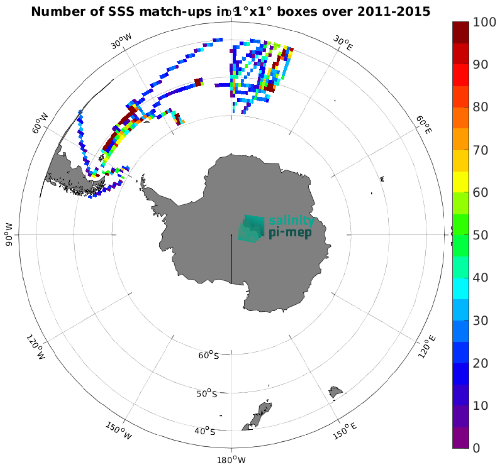
Figure 5: Number of SSS match-ups between TSG (Polarstern) SSS and the Aquarius SSS L3 CAP v5 - 7-Day running (JPL) SSS product for the Roaring Forties and Furious Fifties Pi-MEP region over 1^\circ \times 1^\circ boxes and for the full satellite product period.
