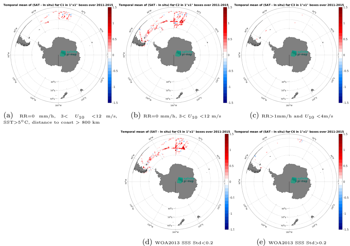
Figure 14: Temporal mean gridded over spatial boxes of size 1^\circ \times 1^\circ of \Delta SSS (Aquarius SSS L3 CAP v5 - 7-Day running (JPL) - TSG (Polarstern)) for 5 different subdatasets corresponding to:RR=0 mm/h, 3 < U_{10} < 12 m/s, SST >5^\circ C, distance to coast > 800 km (a), RR=0 mm/h, 3 < U_{10} < 12 m/s (b), RR >1 mm/h and U_{10} < 4 m/s (c), WOA2013 SSS Std <0.2 (d), WOA2013 SSS Std >0.2 (e).
