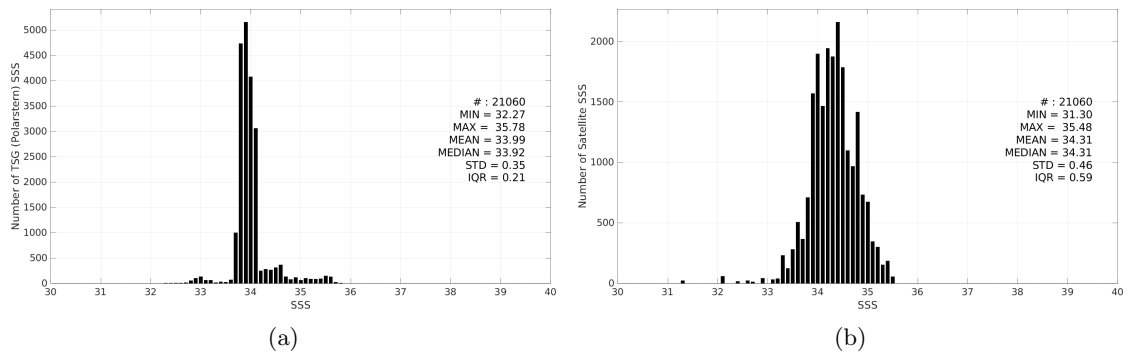
Figure 3: Histograms of SSS from TSG (Polarstern) (a) and Aquarius SSS L3 CAP v5 - 7-Day running (JPL) (b) considering all match-up pairs per bins of 0.1 over the Roaring Forties and Furious Fifties Pi-MEP region and for the full satellite product period.
