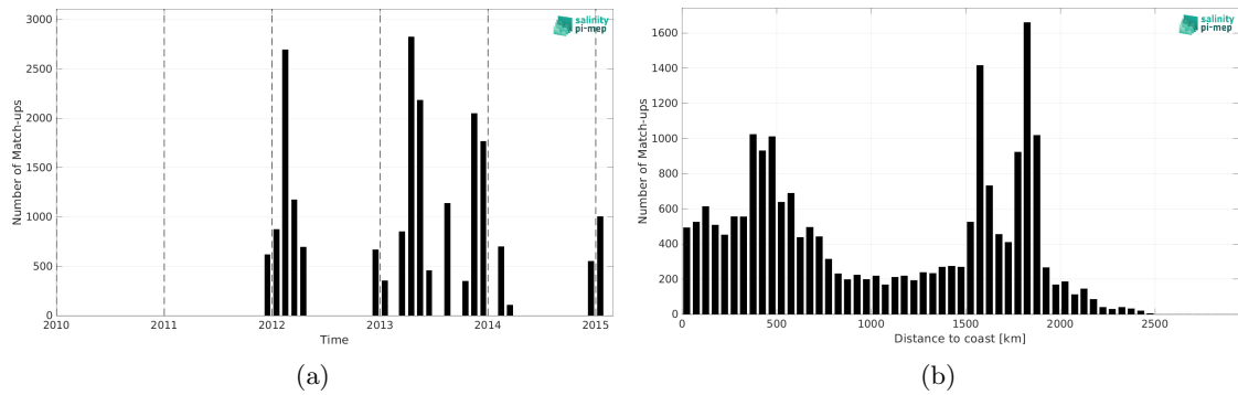
Figure 2: Number of match-ups between TSG (Polarstern) and Aquarius SSS L3 CAP v5 - 7-Day running (JPL) SSS as a function of time (a) and as function of the distance to coast (b) over the Roaring Forties and Furious Fifties Pi-MEP region and for the full satellite product period.
