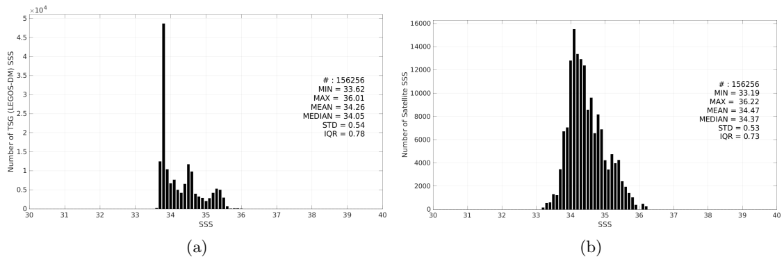
Figure 3: Histograms of SSS from TSG (LEGOS-DM) (a) and Aquarius SSS L3 CAP v5 - 7-Day running (JPL) (b) considering all match-up pairs per bins of 0.1 over the Roaring Forties and Furious Fifties Pi-MEP region and for the full satellite product period.
