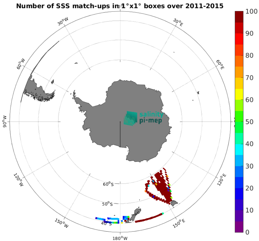
Figure 5: Number of SSS match-ups between TSG (LEGOS-DM) SSS and the Aquarius SSS L3 CAP v5 - 7-Day running (JPL) SSS product for the Roaring Forties and Furious Fifties Pi-MEP region over 1^\circ \times 1^\circ boxes and for the full satellite product period.
