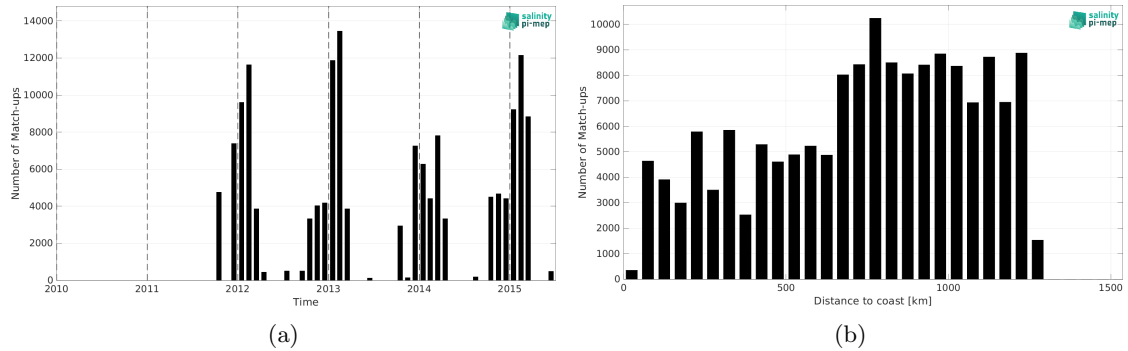
Figure 2: Number of match-ups between TSG (LEGOS-DM) and Aquarius SSS L3 CAP v5 - 7-Day running (JPL) SSS as a function of time (a) and as function of the distance to coast (b) over the Roaring Forties and Furious Fifties Pi-MEP region and for the full satellite product period.
