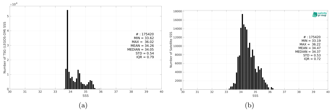
Figure 2: Histograms of SSS from TSG (LEGOS-DM) (a) and Aquarius SSS L3 CAP v5 - 7-Day running (JPL) (b) considering all match-up pairs per bins of 0.1 over the Roaring Forties and Furious Fifties Pi-MEP region and for the full satellite product period.
