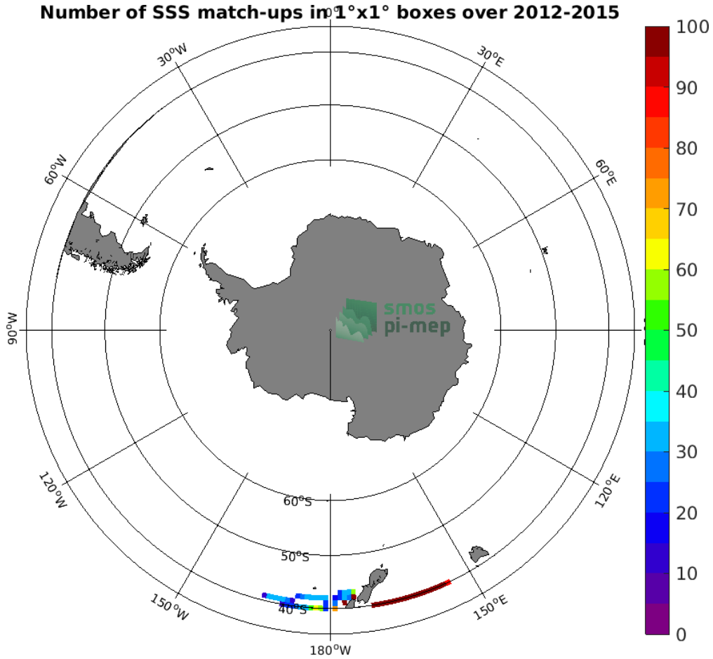
Figure 4: Number of SSS match-ups between TSG (LEGOS-DM) SSS and the Aquarius SSS L3 CAP v5 - 7-Day running (JPL) SSS product for the Roaring Forties and Furious Fifties Pi-MEP region over 1°x1° boxes and for the full satellite product period.
