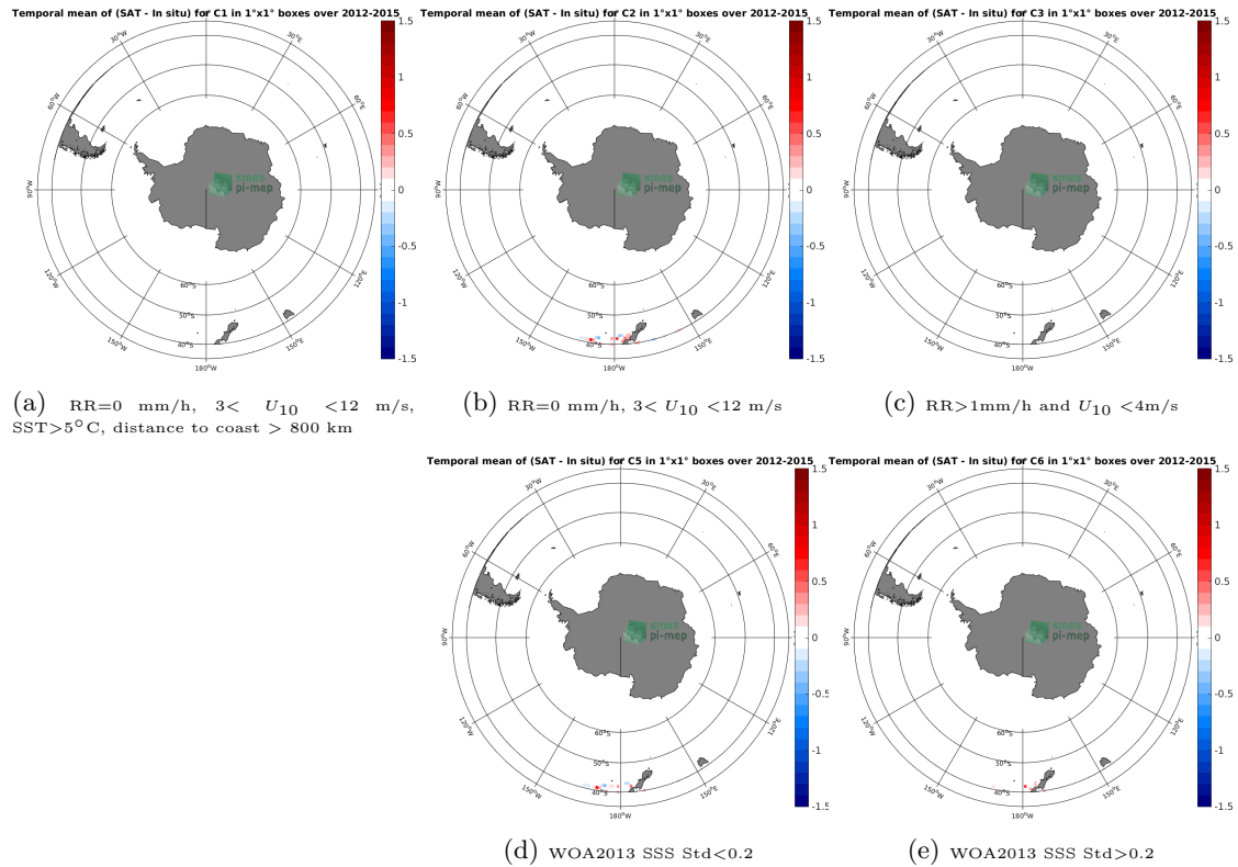
Figure 12: Temporal mean gridded over spatial boxes of size 1^{\circ}\times 1^{\circ} of \Delta\text{SSS} (Aquarius-L3-JPL-V5-7DAY-RUNNING - TSG-LEGOS-DM) for 5 different subdatasets corresponding to:RR=0 mm/h, 3 < U_{10} < 12 m/s, SST >5^{\circ}\text{C} , distance to coast > 800 km (a), RR=0 mm/h, 3 < U_{10} < 12 m/s (b), RR >1 mm/h and U_{10} < 4 m/s (c), WOA2013 SSS Std <0.2 (d), WOA2013 SSS Std >0.2 (e).
