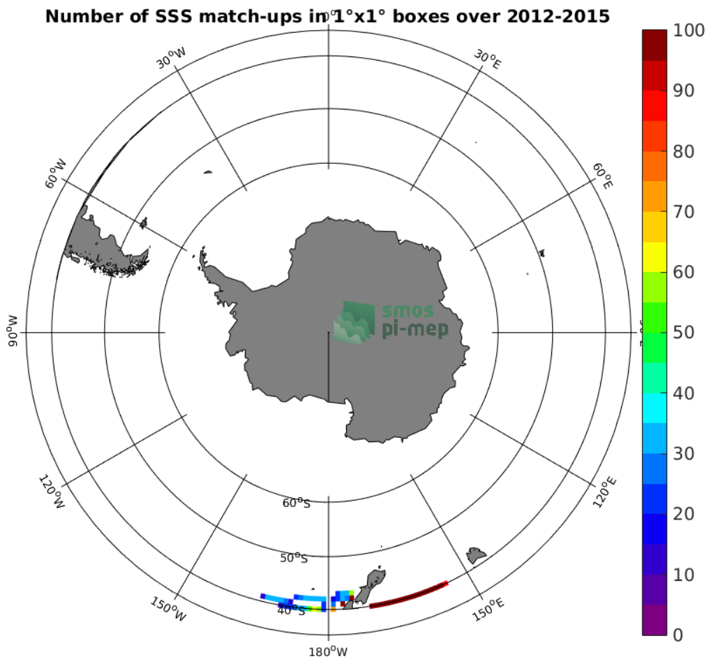
Figure 4: Number of SSS match-ups between TSG-LEGOS-DM SSS and the Aquarius-L3-JPL-V5-7DAY-RUNNING SSS product for the Roaring Forties and Furious Fifties Pi-MEP region over 1^\circ \times 1^\circ boxes and for the full satellite product period.
