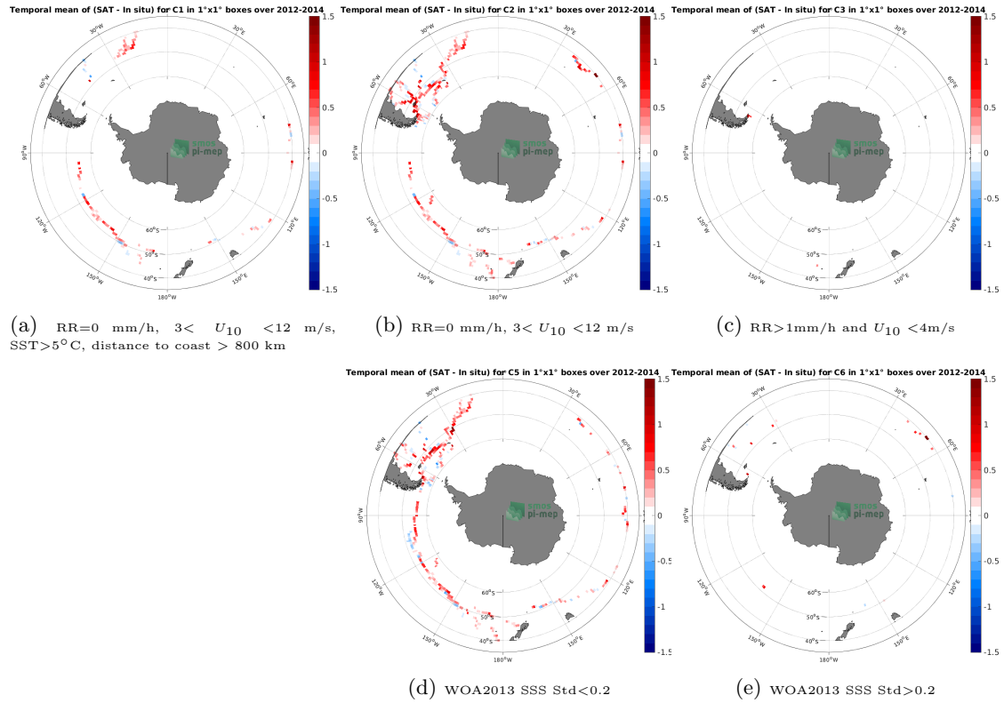
Figure 12: Temporal mean gridded over spatial boxes of size 1^\circ \times 1^\circ of \Delta\text{SSS} (Aquarius SSS L3 CAP v5 - 7-Day running (JPL) - TSG (GOSUD-Sailing-ship)) for 5 different subdatasets corresponding to: RR=0 mm/h, 3 < U_{10} < 12 m/s, SST > 5^\circ\text{C} , distance to coast > 800 km (a), RR=0 mm/h, 3 < U_{10} < 12 m/s (b), RR > 1 mm/h and U_{10} < 4 m/s (c), WOA2013 SSS Std < 0.2 (d), WOA2013 SSS Std > 0.2 (e).
