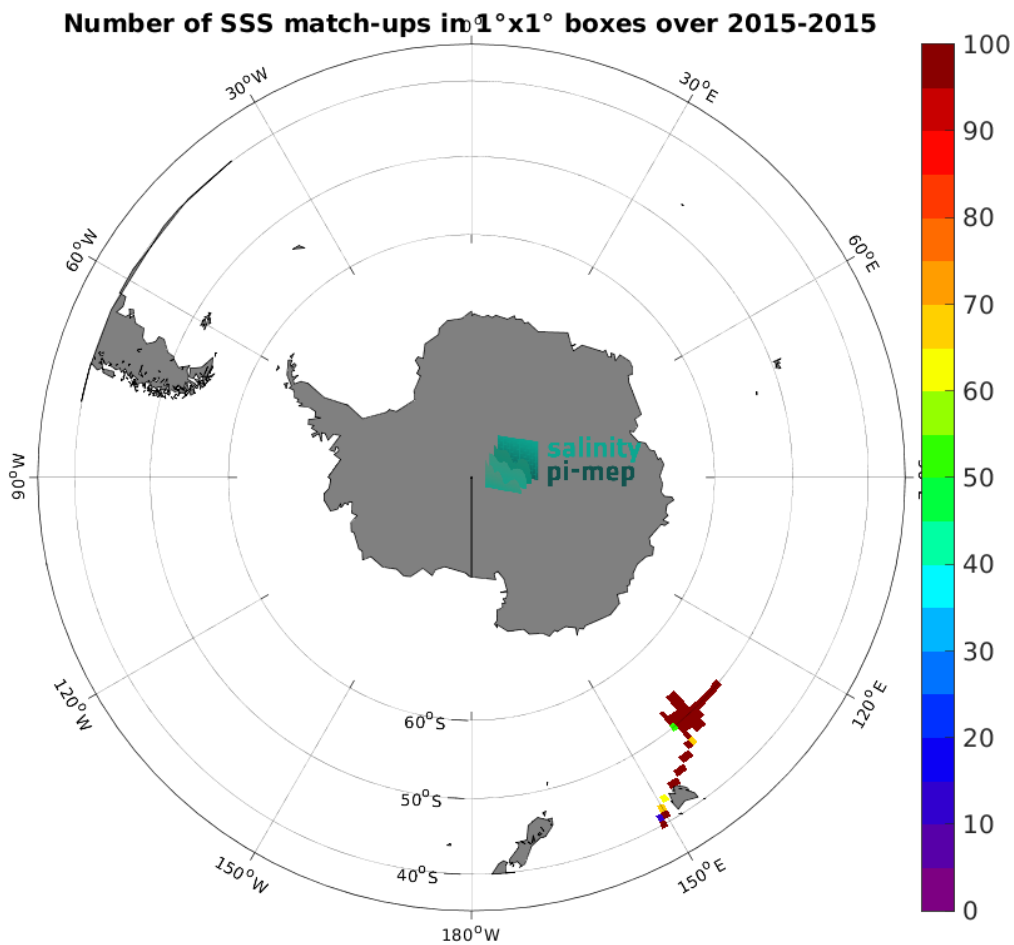
Figure 5: Number of SSS match-ups between TSG (GOSUD-Research-vessel) SSS and the Aquarius SSS L3 CAP v5 - 7-Day running (JPL) SSS product for the Roaring Forties and Furious Fifties Pi-MEP region over 1^\circ \times 1^\circ boxes and for the full satellite product period.
