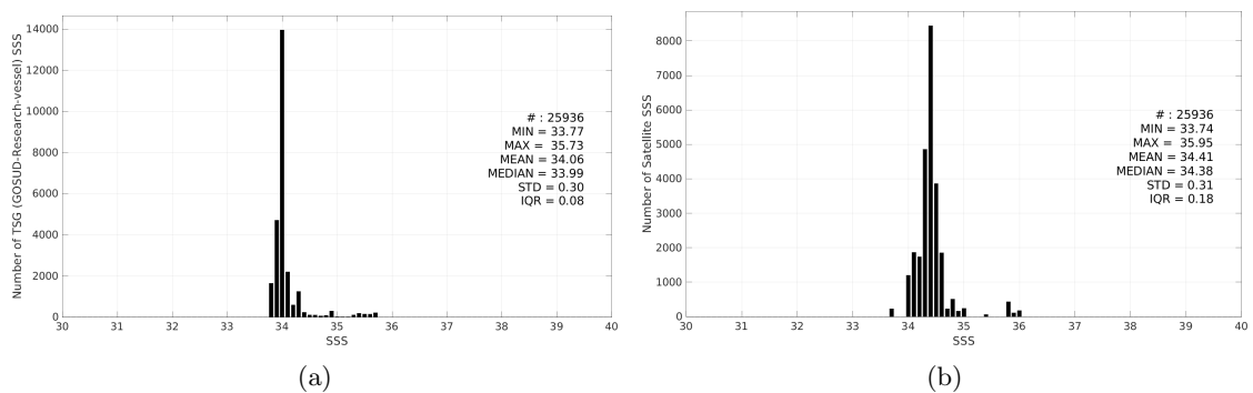
Figure 3: Histograms of SSS from TSG (GOSUD-Research-vessel) (a) and Aquarius SSS L3 CAP v5 - 7-Day running (JPL) (b) considering all match-up pairs per bins of 0.1 over the Roaring Forties and Furious Fifties Pi-MEP region and for the full satellite product period.
