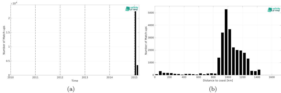
Figure 2: Number of match-ups between TSG (GOSUD-Research-vessel) and Aquarius SSS L3 CAP v5 - 7-Day running (JPL) SSS as a function of time (a) and as function of the distance to coast (b) over the Roaring Forties and Furious Fifties Pi-MEP region and for the full satellite product period.
