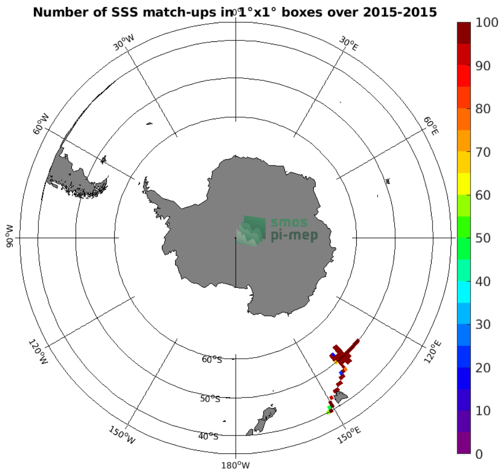
Figure 4: Number of SSS match-ups between TSG (GOSUD-Research-vessel) SSS and the Aquarius SSS L3 CAP v5 - 7-Day running (JPL) SSS product for the Roaring Forties and Furious Fifties Pi-MEP region over 1^\circ \times 1^\circ boxes and for the full satellite product period.
