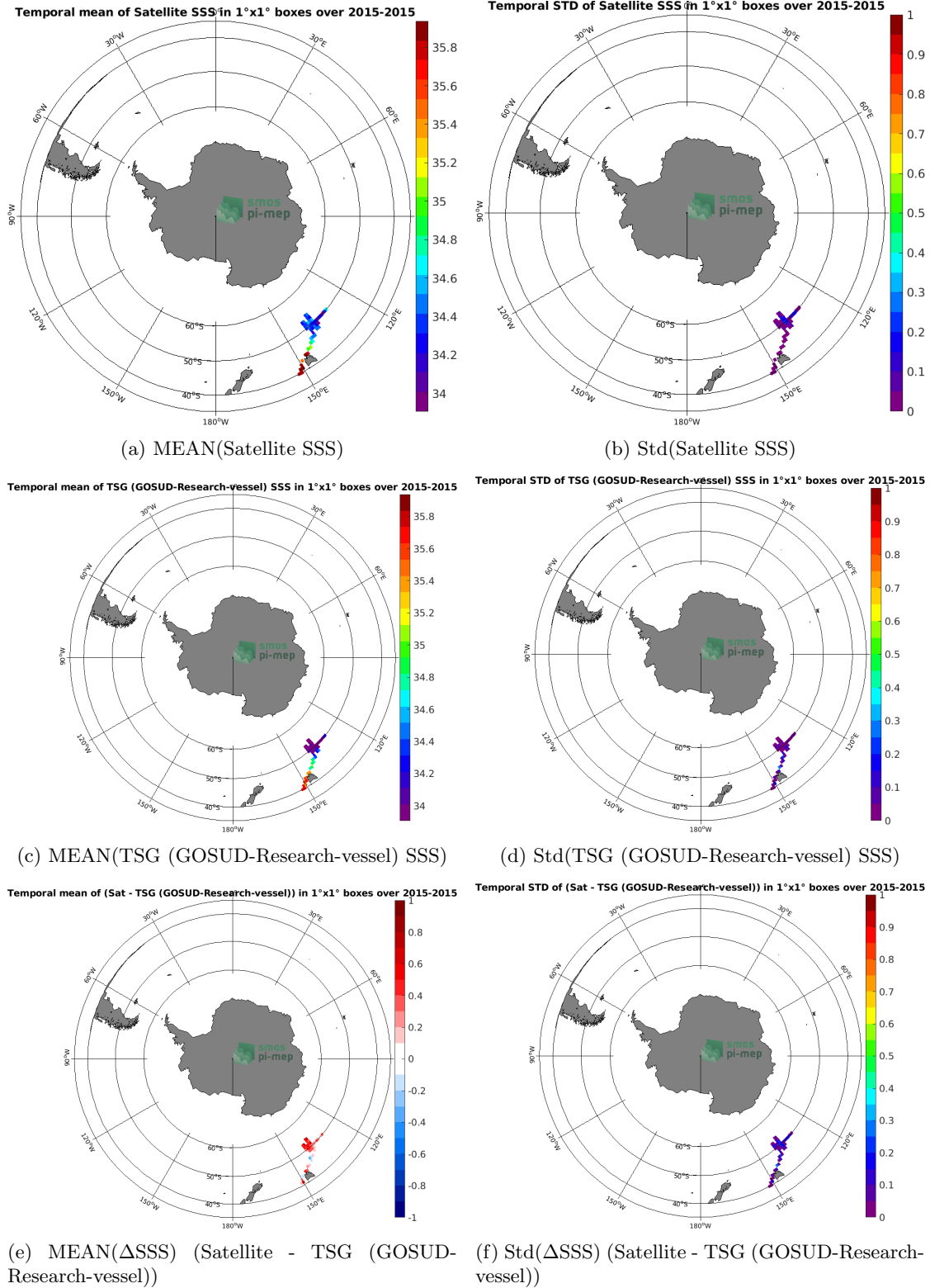
Figure 6: Temporal mean (left) and Std (right) of SSS from Aquarius SSS L3 CAP v5 - 7-Day running (JPL) (top), TSG (GOSUD-Research-vessel) (middle), and of \Delta SSS (Satellite - TSG (GOSUD-Research-vessel)). Only match-up pairs are used to generate these maps.
