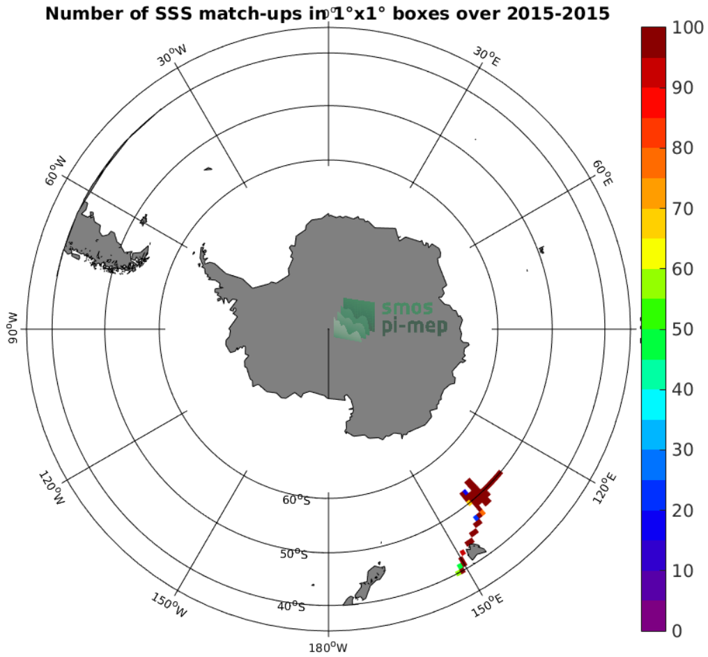
Figure 4: Number of SSS match-ups between TSG-GOSUD-Research-vessel SSS and the Aquarius-L3-JPL-V5-7DAY-RUNNING SSS product for the Roaring Forties and Furious Fifties Pi-MEP region over 1^{\circ} \times 1^{\circ} boxes and for the full satellite product period.
