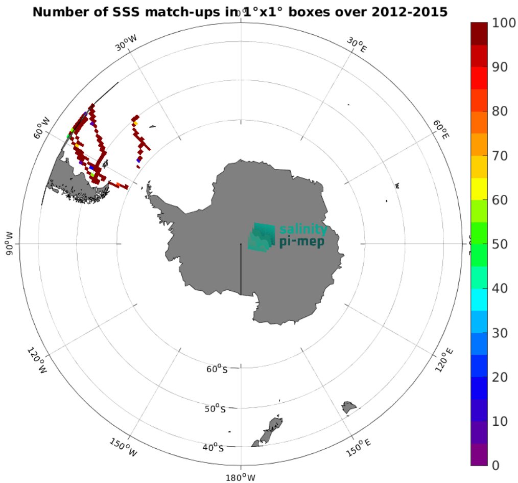
Figure 4: Number of SSS match-ups between TSG (CSIC-UTM) SSS and the Aquarius SSS L3 CAP v5 - 7-Day running (JPL) SSS product for the Roaring Forties and Furious Fifties Pi-MEP region over 1^{\circ} \times 1^{\circ} boxes and for the full satellite product period.
