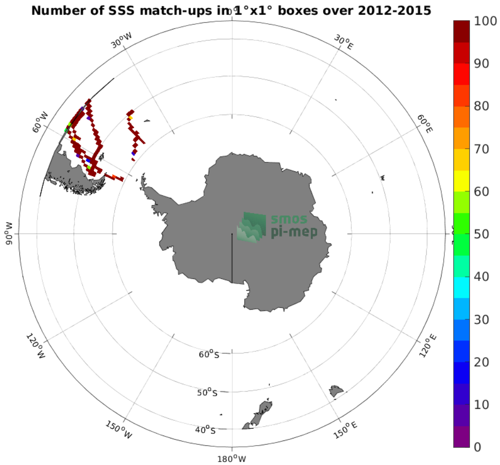
Figure 4: Number of SSS match-ups between TSG (CSIC-UTM) SSS and the Aquarius SSS L3 CAP v5 - 7-Day running (JPL) SSS product for the Roaring Forties and Furious Fifties Pi-MEP region over 1^\circ \times 1^\circ boxes and for the full satellite product period.
