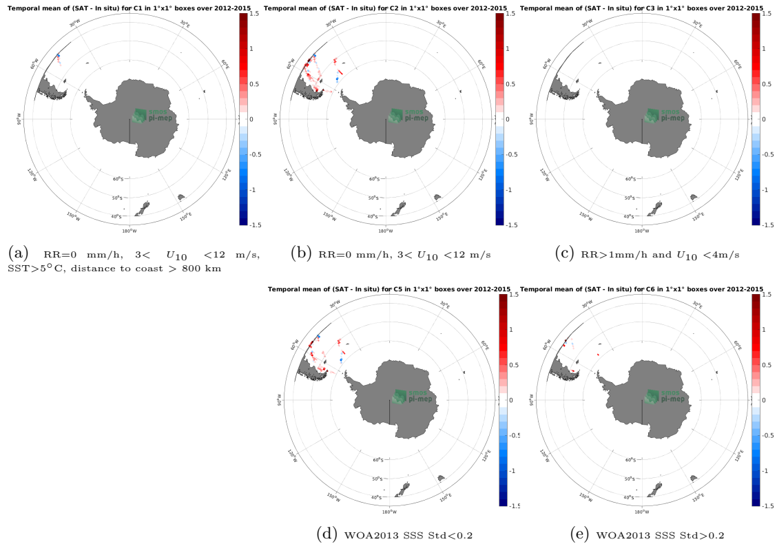
Figure 12: Temporal mean gridded over spatial boxes of size 1^{\circ}\times 1^{\circ} of \Delta\text{SSS} (Aquarius SSS L3 CAP v5 - 7-Day running (JPL) - TSG (CSIC-UTM)) for 5 different subdatasets corresponding to:RR=0 mm/h, 3 < U_{10} < 12 m/s, SST >5^{\circ}\text{C} , distance to coast > 800 km (a), RR=0 mm/h, 3 < U_{10} < 12 m/s (b), RR >1 mm/h and U_{10} < 4 m/s (c), WOA2013 SSS Std <0.2 (d), WOA2013 SSS Std >0.2 (e).
