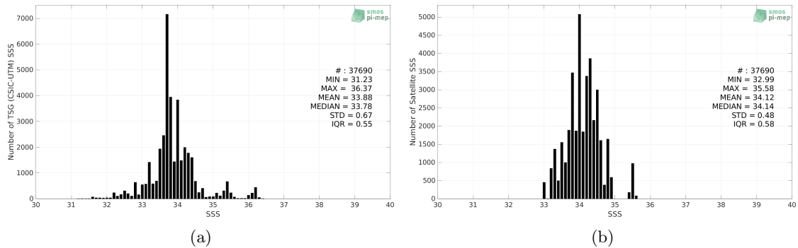
Figure 2: Histograms of SSS from TSG (CSIC-UTM) (a) and Aquarius SSS L3 CAP v5 - 7-Day running (JPL) (b) considering all match-up pairs per bins of 0.1 over the Roaring Forties and Furious Fifties Pi-MEP region and for the full satellite product period.
