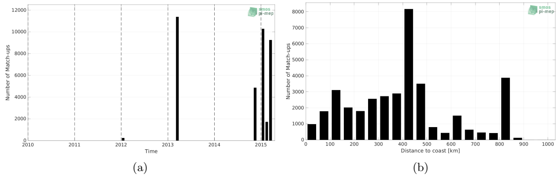
Figure 1: Number of match-ups between TSG (CSIC-UTM) and Aquarius SSS L3 CAP v5 - 7-Day running (JPL) SSS as a function of time (a) and as function of the distance to coast (b) over the Roaring Forties and Furious Fifties Pi-MEP region and for the full satellite product period.
