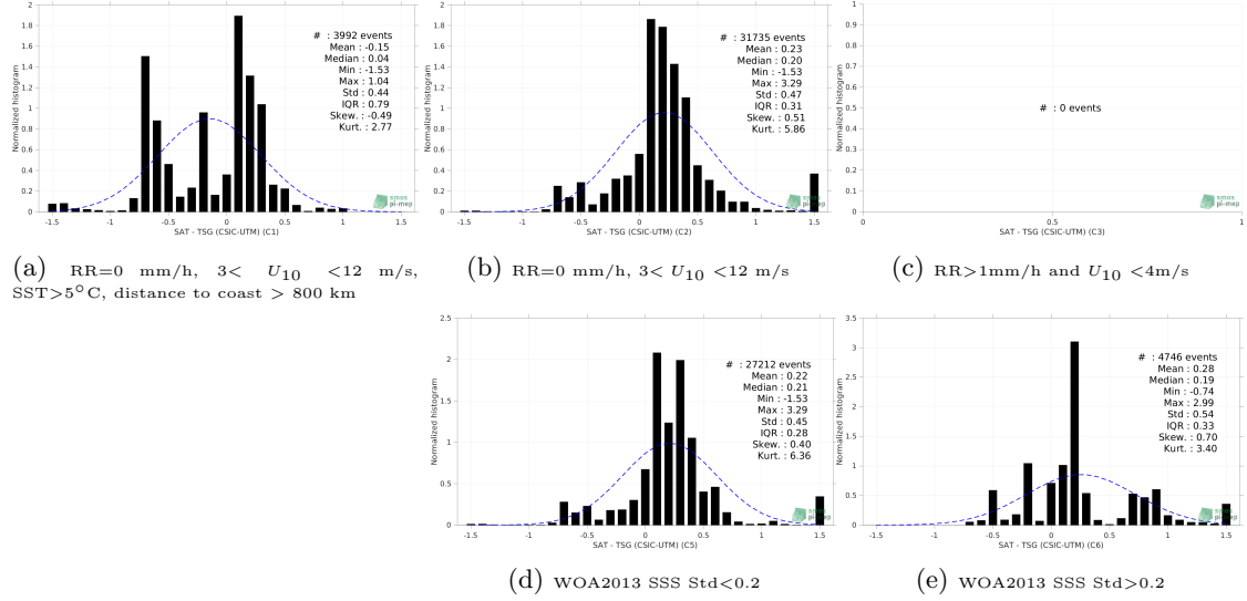
Figure 13: Normalized histogram of \Delta SSS (Aquarius SSS L3 CAP v5 - 7-Day running (JPL) - TSG (CSIC-UTM)) for 5 different subdatasets corresponding to: RR=0 mm/h, 3 < U_{10} < 12 m/s, SST>5°C, distance to coast > 800 km (a), RR=0 mm/h, 3 < U_{10} < 12 m/s (b), RR>1mm/h and U_{10} < 4 m/s (c), WOA2013 SSS Std<0.2 (d), WOA2013 SSS Std>0.2 (e).
