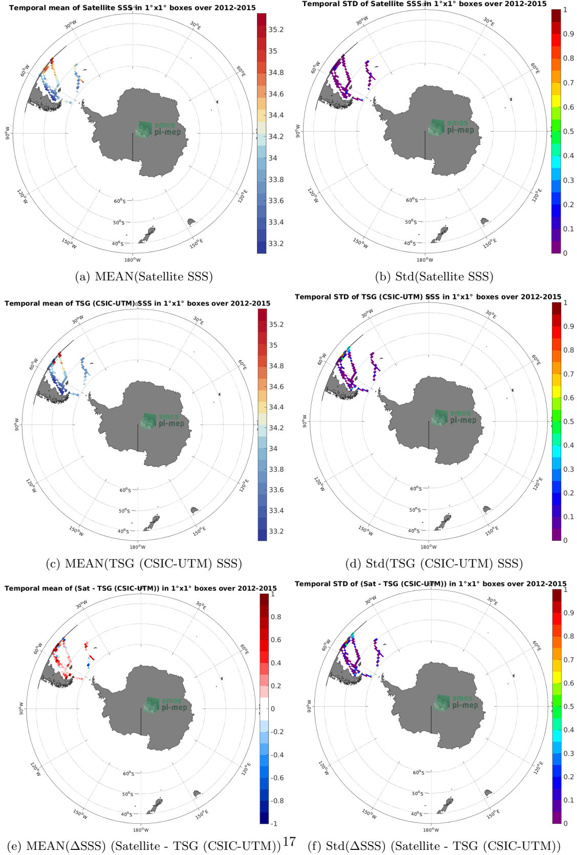
Figure 6: Temporal mean (left) and Std (right) of SSS from Aquarius SSS L3 CAP v5 - 7-Day running (JPL) (top), TSG (CSIC-UTM) (middle), and of \Delta SSS (Satellite - TSG (CSIC-UTM)). Only match-up pairs are used to generate these maps.
