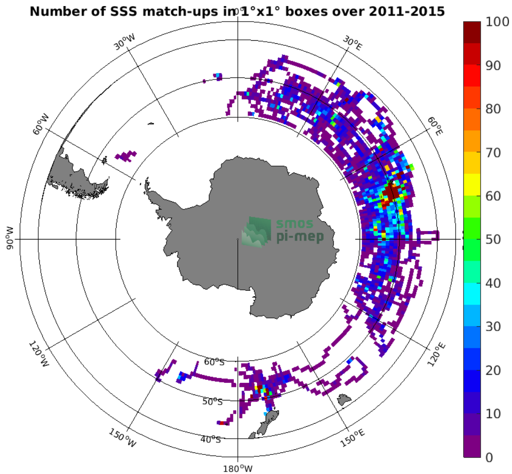
Figure 4: Number of SSS match-ups between Sea mammals SSS and the Aquarius SSS L3 CAP v5 - 7-Day running (JPL) SSS product for the Roaring Forties and Furious Fifties Pi-MEP region over 1°x1° boxes and for the full satellite product period.
