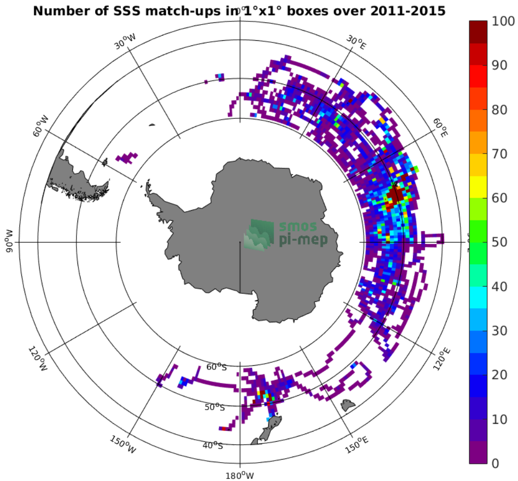
Figure 4: Number of SSS match-ups between Sea mammals SSS and the Aquarius-L3-JPL-V5-7DAY-RUNNING SSS product for the Roaring Forties and Furious Fifties Pi-MEP region over 1^\circ \times 1^\circ boxes and for the full satellite product period.
