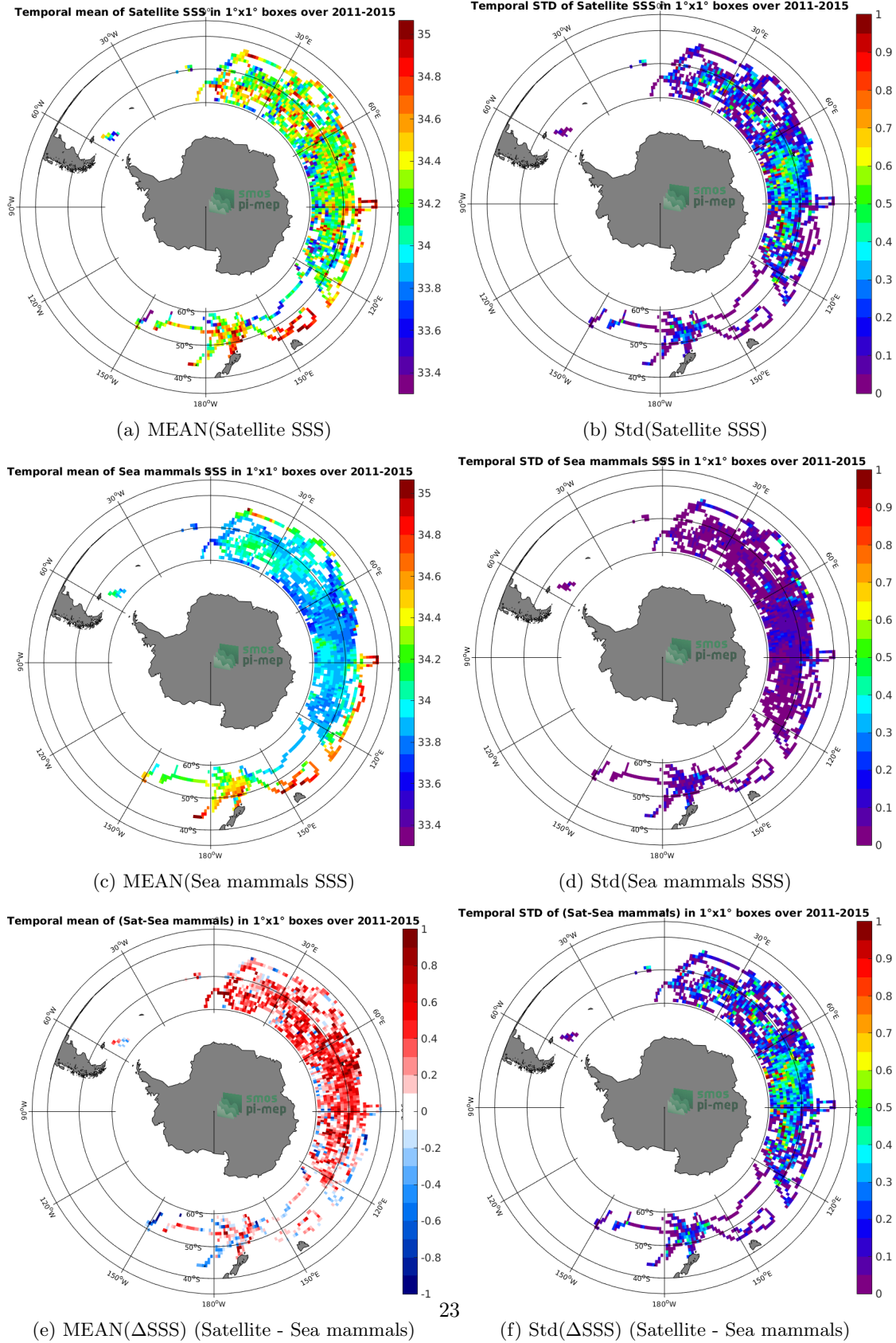
Figure 6: Temporal mean (left) and Std (right) of SSS from Aquarius-L3-JPL-V5-7DAY-RUNNING (top), Sea mammals (middle), and of \Delta SSS (Satellite - Sea mammals). Only match-up pairs are used to generate these maps.
