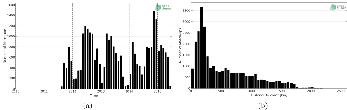
Figure 1: Number of match-ups between Sea mammals and Aquarius-L3-JPL-V5-7DAY-RUNNING SSS as a function of time (a) and as function of the distance to coast (b) over the Roaring Forties and Furious Fifties Pi-MEP region and for the full satellite product period.
