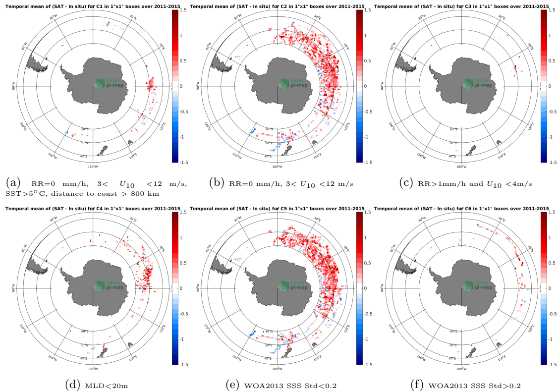
Figure 12: Temporal mean gridded over spatial boxes of size 1^\circ \times 1^\circ of \Delta SSS (Aquarius-L3-JPL-V5-7DAY-RUNNING - Sea mammals) for 6 different subdatasets corresponding to:RR=0 mm/h, 3 < U_{10} < 12 m/s, SST >5^\circ C, distance to coast > 800 km (a), RR=0 mm/h, 3 < U_{10} < 12 m/s (b), RR >1 mm/h and U_{10} < 4 m/s (c),MLD <20 m (d),WOA2013 SSS Std <0.2 (e),WOA2013 SSS Std >0.2 (f).
