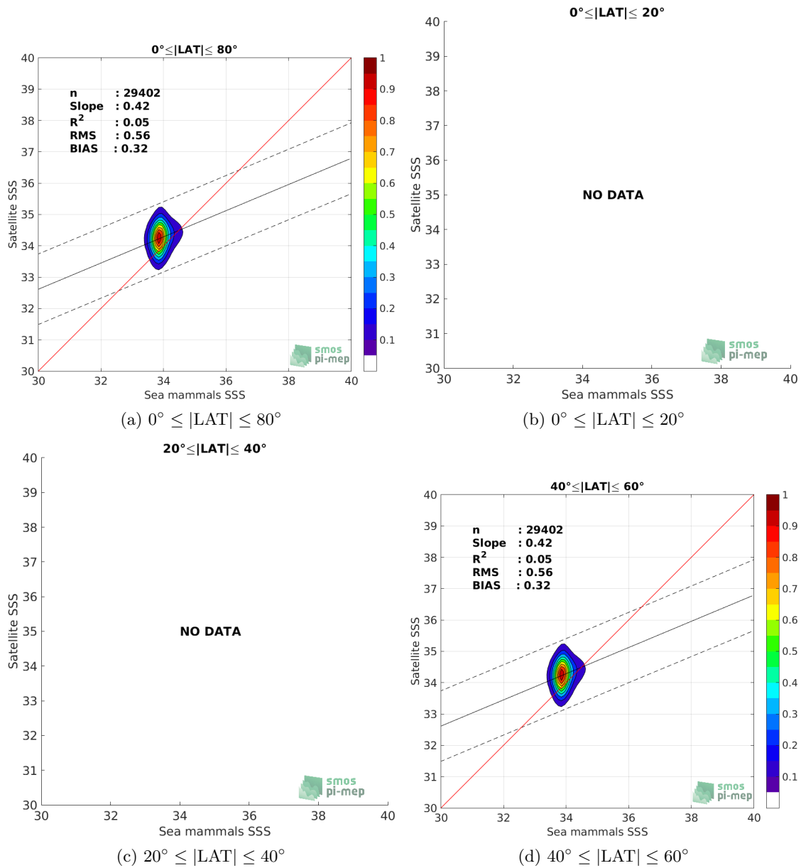
Figure 9: Contour maps of the concentration of Aquarius-L3-JPL-V5-7DAY-RUNNING SSS (y-axis) versus Sea mammals SSS (x-axis) at match-up pairs for different latitude bands. For each plot, the red line shows x=y . The black thin and dashed lines indicate a linear fit through the data cloud and the \pm 95\% confidence levels, respectively. The number match-up pairs n , the slope and R^2 coefficient of the linear fit, the root mean square (RMS) and the mean bias between satellite and in situ data are indicated for each latitude band in each plots.
