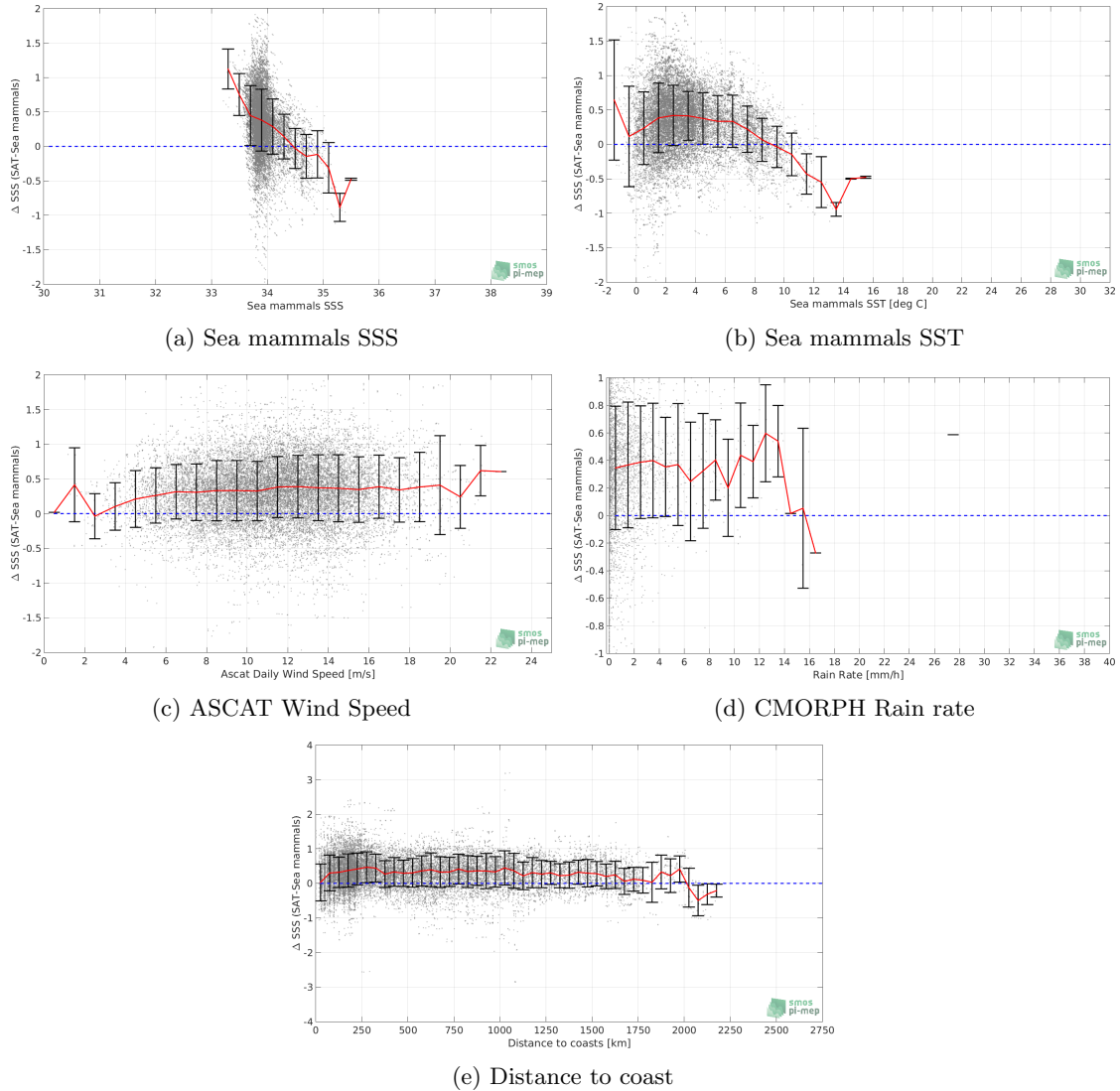
Figure 11: \Delta SSS (Satellite - Sea mammals) sorted as function of Sea mammals SSS values a), Sea mammals SST b), ASCAT Wind speed c), CMORPH rain rate d) and distance to coast (e). In all plots the mean and Std of \Delta SSS for each bin is indicated by the red curves and black vertical thick bars ( \pm 1 Std)
