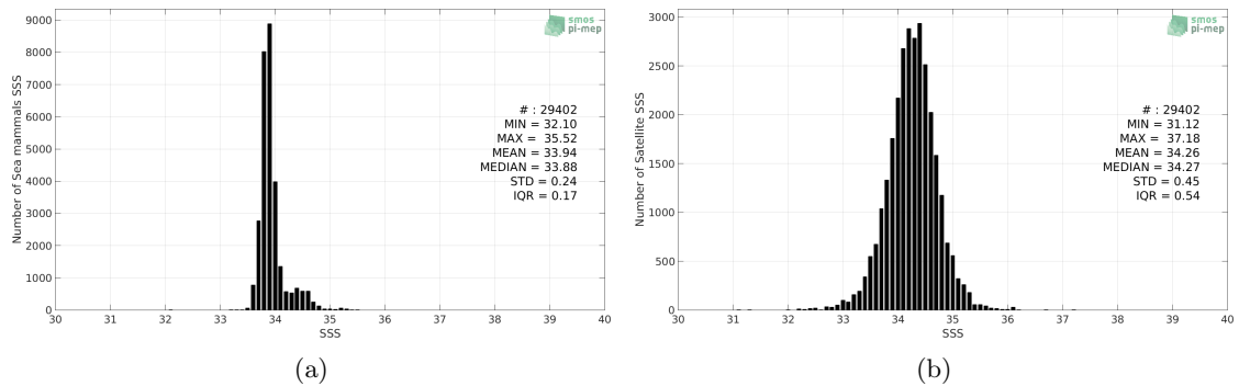
Figure 2: Histograms of SSS from Sea mammals (a) and Aquarius-L3-JPL-V5-7DAY-RUNNING (b) considering all match-up pairs per bins of 0.1 over the Roaring Forties and Furious Fifties Pi-MEP region and for the full satellite product period.
