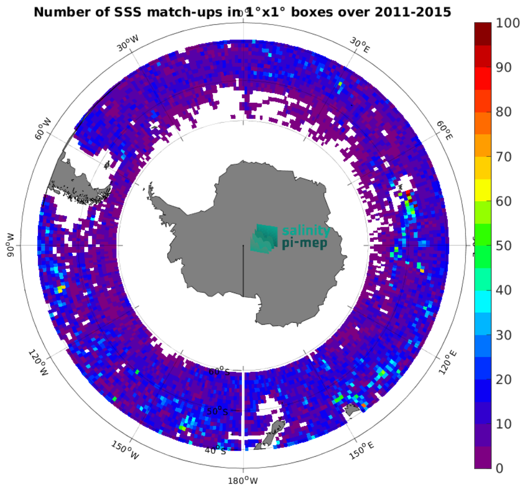
Figure 5: Number of SSS match-ups between Argo SSS and the Aquarius SSS L3 CAP v5 - 7-Day running (JPL) SSS product for the Roaring Forties and Furious Fifties Pi-MEP region over 1^{\circ} \times 1^{\circ} boxes and for the full satellite product period.
