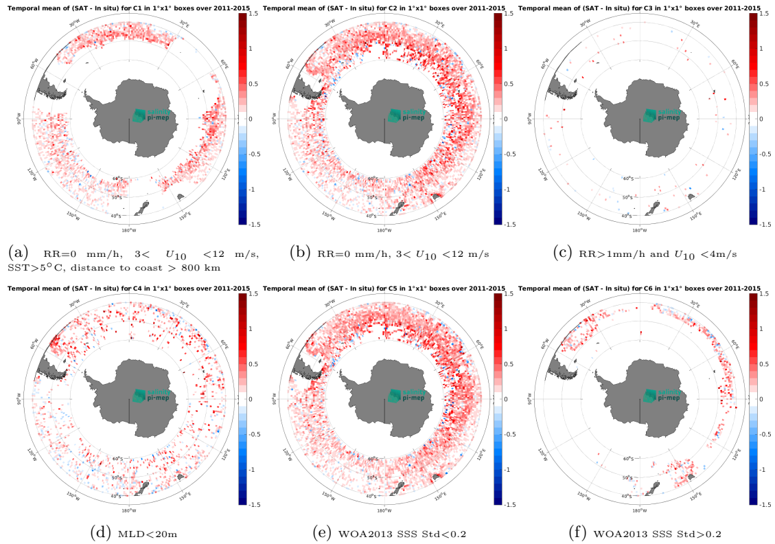
Figure 14: Temporal mean gridded over spatial boxes of size 1^\circ \times 1^\circ of \Delta\text{SSS} (Aquarius SSS L3 CAP v5 - 7-Day running (JPL) - Argo) for 6 different subdatasets corresponding to:RR=0 mm/h, 3 < U_{10} < 12 m/s, SST>5°C, distance to coast > 800 km (a), RR=0 mm/h, 3 < U_{10} < 12 m/s (b), RR>1mm/h and U_{10} < 4 m/s (c),MLD<20m (d),WOA2013 SSS Std<0.2 (e),WOA2013 SSS Std>0.2 (f).
