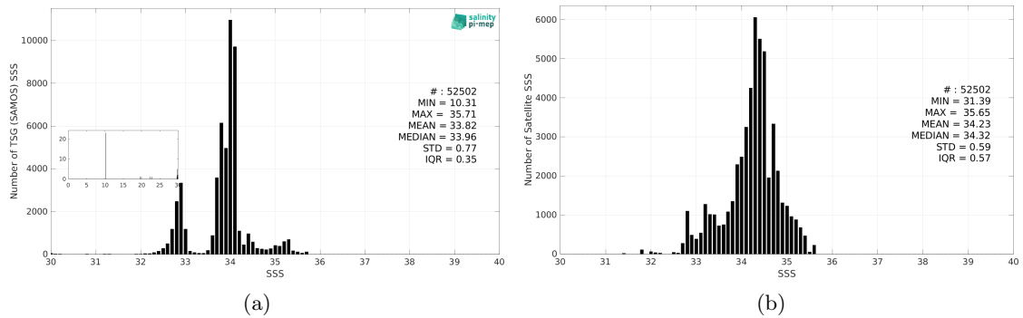
Figure 3: Histograms of SSS from TSG (SAMOS) (a) and Aquarius SSS L3 CAP v5 - Monthly (JPL) (b) considering all match-up pairs per bins of 0.1 over the Roaring Forties and Furious Fifties Pi-MEP region and for the full satellite product period.
