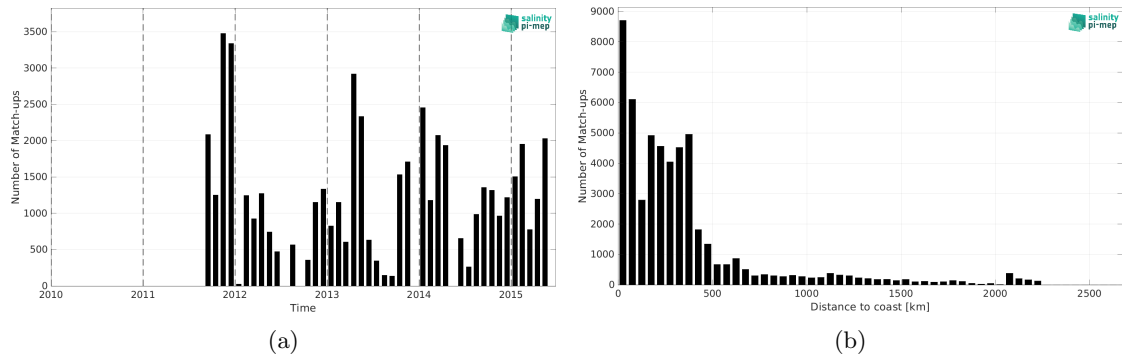
Figure 2: Number of match-ups between TSG (SAMOS) and Aquarius SSS L3 CAP v5 - Monthly (JPL) SSS as a function of time (a) and as function of the distance to coast (b) over the Roaring Forties and Furious Fifties Pi-MEP region and for the full satellite product period.
