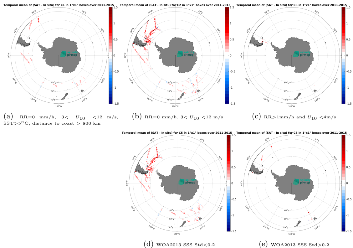
Figure 14: Temporal mean gridded over spatial boxes of size 1^\circ \times 1^\circ of \Delta SSS (Aquarius SSS L3 CAP v5 - Monthly (JPL) - TSG (SAMOS)) for 5 different subdatasets corresponding to:RR=0 mm/h, 3 < U_{10} < 12 m/s, SST > 5^\circ\text{C} , distance to coast > 800 km (a), RR=0 mm/h, 3 < U_{10} < 12 m/s (b), RR > 1 mm/h and U_{10} < 4 m/s (c), WOA2013 SSS Std < 0.2 (d), WOA2013 SSS Std > 0.2 (e).
