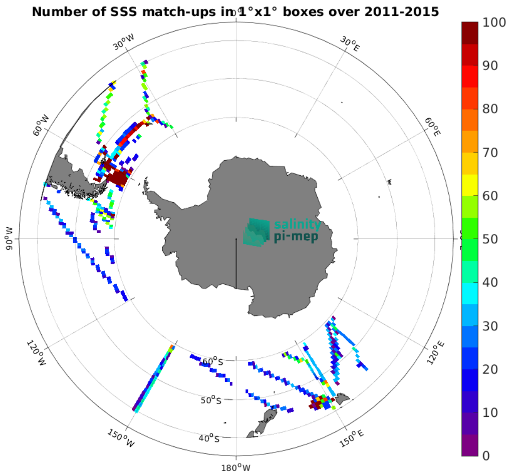
Figure 5: Number of SSS match-ups between TSG (SAMOS) SSS and the Aquarius SSS L3 CAP v5 - Monthly (JPL) SSS product for the Roaring Forties and Furious Fifties Pi-MEP region over 1^\circ \times 1^\circ boxes and for the full satellite product period.
