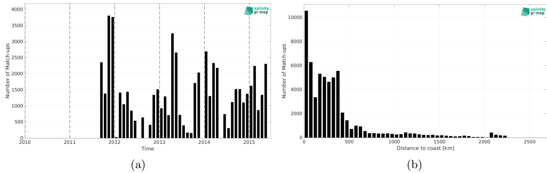
Figure 1: Number of match-ups between TSG (SAMOS) and Aquarius SSS L3 CAP v5 - Monthly (JPL) SSS as a function of time (a) and as function of the distance to coast (b) over the Roaring Forties and Furious Fifties Pi-MEP region and for the full satellite product period.
