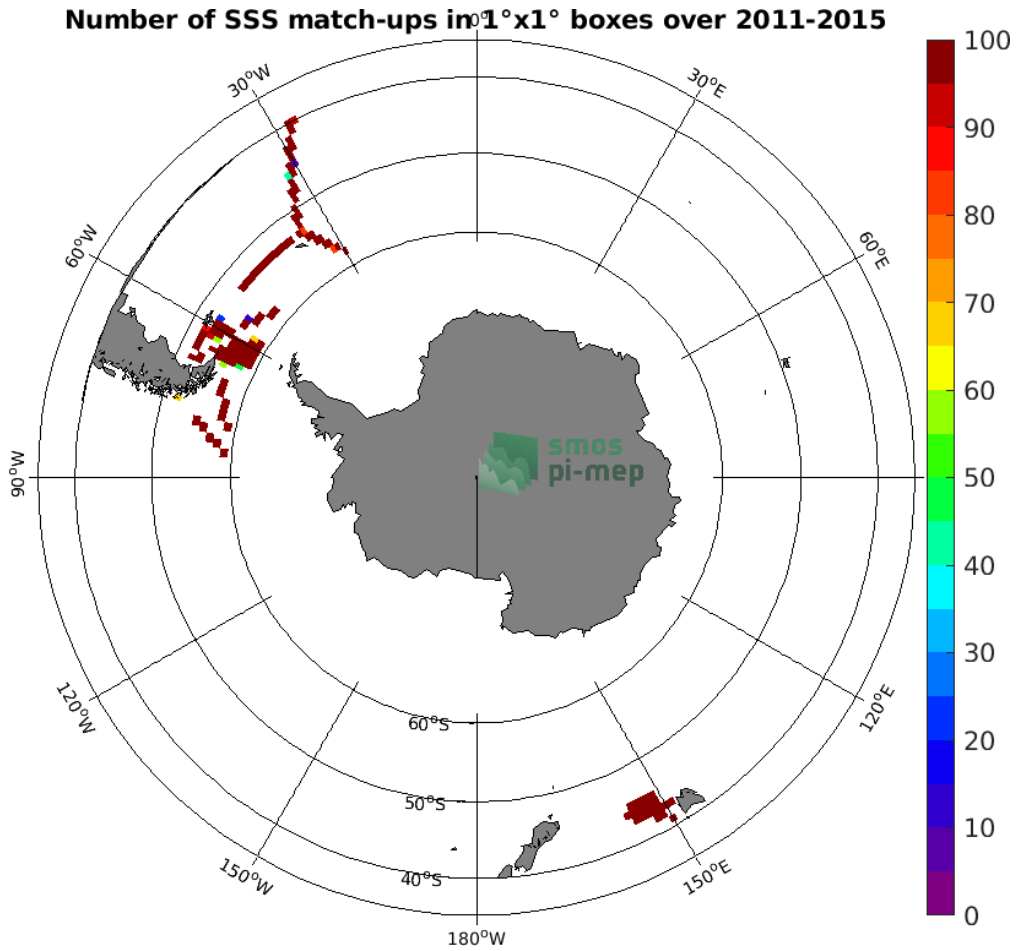
Figure 4: Number of SSS match-ups between TSG (SAMOS) SSS and the Aquarius SSS L3 CAP v5 - Monthly (JPL) SSS product for the Roaring Forties and Furious Fifties Pi-MEP region over 1°x1° boxes and for the full satellite product period.
