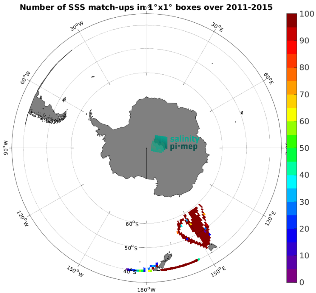
Figure 5: Number of SSS match-ups between TSG (LEGOS-DM) SSS and the Aquarius SSS L3 CAP v5 - Monthly (JPL) SSS product for the Roaring Forties and Furious Fifties Pi-MEP region over 1^{\circ} \times 1^{\circ} boxes and for the full satellite product period.
