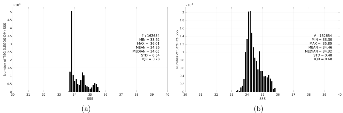
Figure 3: Histograms of SSS from TSG (LEGOS-DM) (a) and Aquarius SSS L3 CAP v5 - Monthly (JPL) (b) considering all match-up pairs per bins of 0.1 over the Roaring Forties and Furious Fifties Pi-MEP region and for the full satellite product period.
