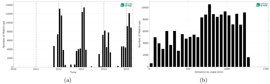
Figure 2: Number of match-ups between TSG (LEGOS-DM) and Aquarius SSS L3 CAP v5 - Monthly (JPL) SSS as a function of time (a) and as function of the distance to coast (b) over the Roaring Forties and Furious Fifties Pi-MEP region and for the full satellite product period.
