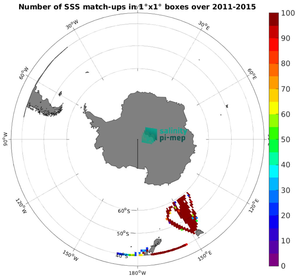
Figure 4: Number of SSS match-ups between TSG (LEGOS-DM) SSS and the Aquarius SSS L3 CAP v5 - Monthly (JPL) SSS product for the Roaring Forties and Furious Fifties Pi-MEP region over 1^{\circ} \times 1^{\circ} boxes and for the full satellite product period.
