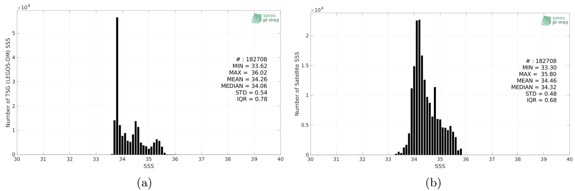
Figure 2: Histograms of SSS from TSG (LEGOS-DM) (a) and Aquarius SSS L3 CAP v5 - Monthly (JPL) (b) considering all match-up pairs per bins of 0.1 over the Roaring Forties and Furious Fifties Pi-MEP region and for the full satellite product period.
