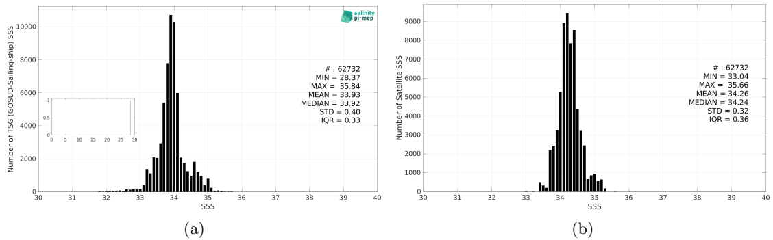
Figure 3: Histograms of SSS from TSG (GOSUD-Sailing-ship) (a) and Aquarius SSS L3 CAP v5 - Monthly (JPL) (b) considering all match-up pairs per bins of 0.1 over the Roaring Forties and Furious Fifties Pi-MEP region and for the full satellite product period.
