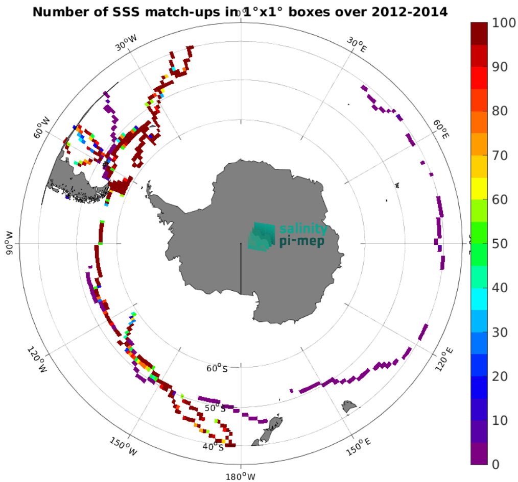
Figure 5: Number of SSS match-ups between TSG (GOSUD-Sailing-ship) SSS and the Aquarius SSS L3 CAP v5 - Monthly (JPL) SSS product for the Roaring Forties and Furious Fifties Pi-MEP region over 1^\circ \times 1^\circ boxes and for the full satellite product period.
