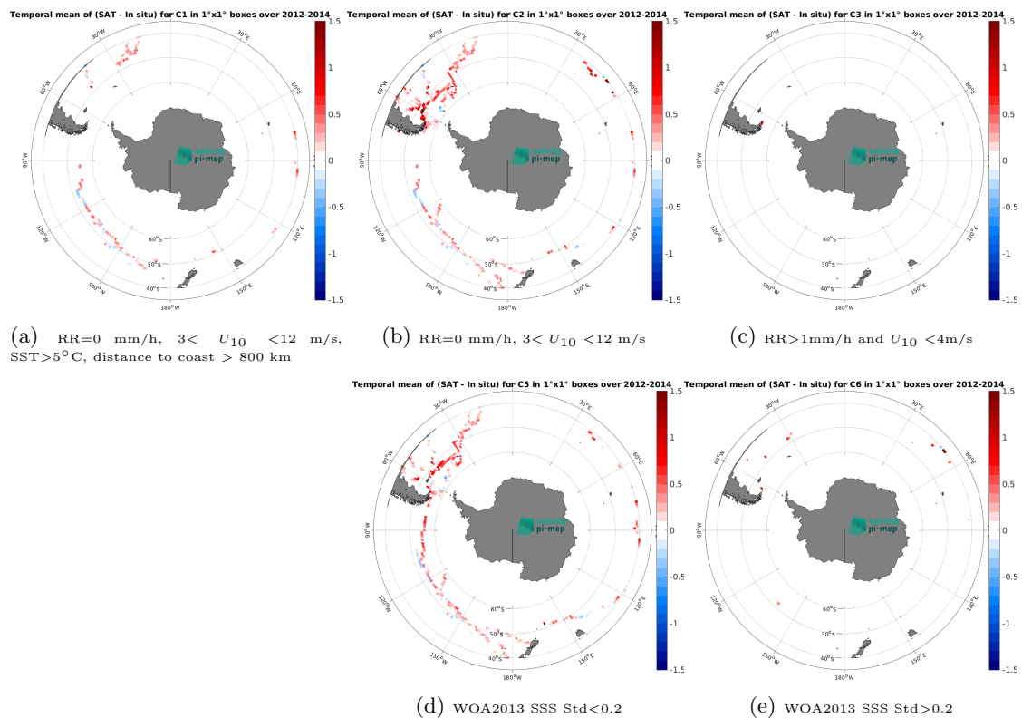
Figure 14: Temporal mean gridded over spatial boxes of size 1^\circ \times 1^\circ of \Delta SSS (Aquarius SSS L3 CAP v5 - Monthly (JPL) - TSG (GOSUD-Sailing-ship)) for 5 different subdatasets corresponding to:RR=0 mm/h, 3 < U_{10} < 12 m/s, SST>5°C, distance to coast > 800 km (a), RR=0 mm/h, 3 < U_{10} < 12 m/s (b), RR>1mm/h and U_{10} < 4 m/s (c), WOA2013 SSS Std<0.2 (d), WOA2013 SSS Std>0.2 (e).
