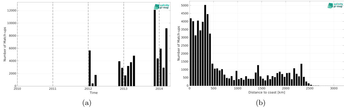
Figure 2: Number of match-ups between TSG (GOSUD-Sailing-ship) and Aquarius SSS L3 CAP v5 - Monthly (JPL) SSS as a function of time (a) and as function of the distance to coast (b) over the Roaring Forties and Furious Fifties Pi-MEP region and for the full satellite product period.
