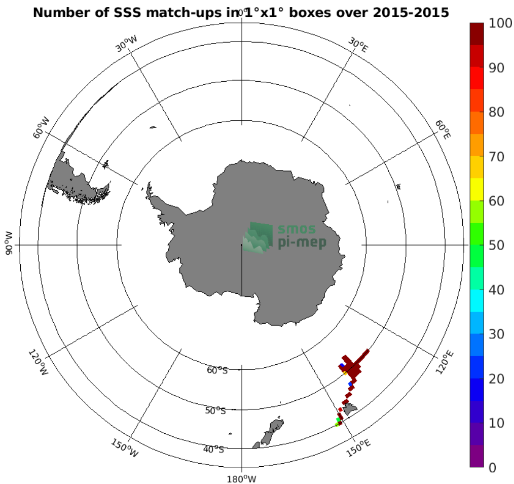
Figure 4: Number of SSS match-ups between TSG (GOSUD-Research-vessel) SSS and the Aquarius SSS L3 CAP v5 - Monthly (JPL) SSS product for the Roaring Forties and Furious Fifties Pi-MEP region over 1^\circ \times 1^\circ boxes and for the full satellite product period.
