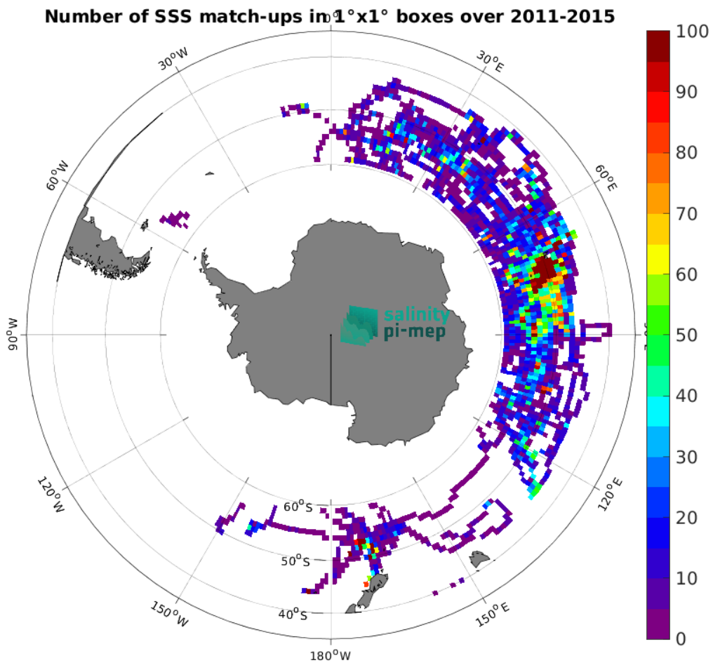
Figure 4: Number of SSS match-ups between Marine mammals SSS and the Aquarius SSS L3 CAP v5 - Monthly (JPL) SSS product for the Roaring Forties and Furious Fifties Pi-MEP region over 1^{\circ} \times 1^{\circ} boxes and for the full satellite product period.
