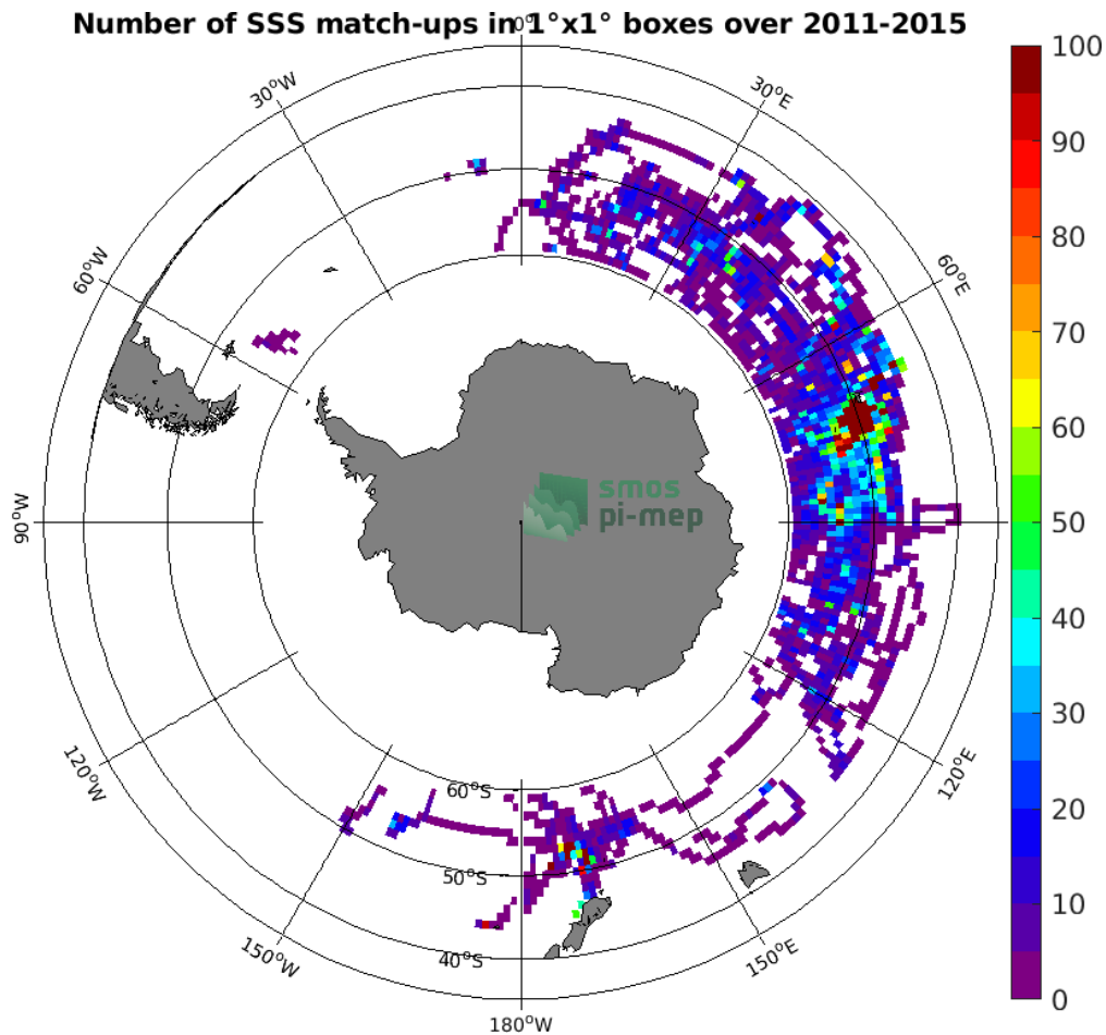
Figure 4: Number of SSS match-ups between Marine mammals SSS and the Aquarius SSS L3 CAP v5 - Monthly (JPL) SSS product for the Roaring Forties and Furious Fifties Pi-MEP region over 1^\circ \times 1^\circ boxes and for the full satellite product period.
