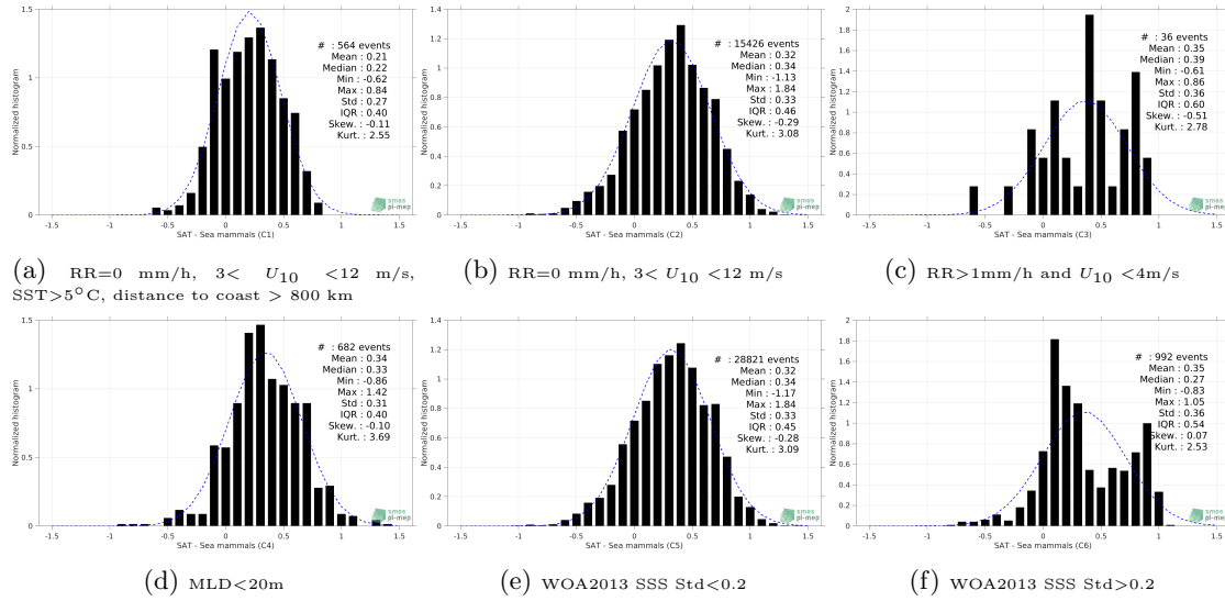
Figure 13: Normalized histogram of \Delta SSS (Aquarius SSS L3 CAP v5 - Monthly (JPL) - Marine mammals) for 6 different subdatasets corresponding to: RR=0 mm/h, 3 < U_{10} < 12 m/s, SST > 5°C, distance to coast > 800 km (a), RR=0 mm/h, 3 < U_{10} < 12 m/s (b), RR > 1mm/h and U_{10} < 4 m/s (c), MLD < 20m (d), WOA2013 SSS Std < 0.2 (e), WOA2013 SSS Std > 0.2 (f).
