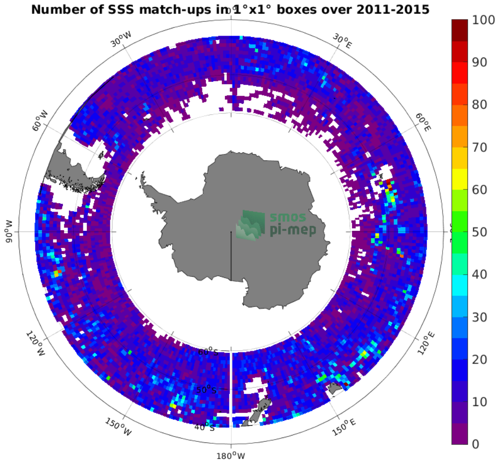
Figure 4: Number of SSS match-ups between Argo SSS and the Aquarius SSS L3 CAP v5 - Monthly (JPL) SSS product for the Roaring Forties and Furious Fifties Pi-MEP region over 1^\circ \times 1^\circ boxes and for the full satellite product period.
