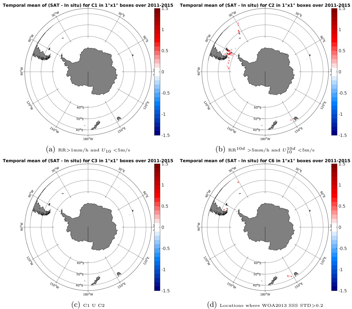
Figure 12: Temporal mean gridded over spatial boxes of size 1^\circ \times 1^\circ of \Delta SSS (Aquarius-L3-JPL-V4-7DAY-RUNNING - TSG-SAMOS) for 4 different subdatasets corresponding to: RR > 1\text{mm/h} and U_{10} < 5\text{m/s} (a), RR^{10d} > 5\text{mm/h} and U_{10}^{10d} < 5\text{m/s} (b), C1 U C2 (c), Locations where WOA2013 SSS STD > 0.2 (d).
