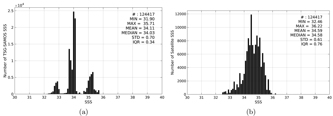
Figure 2: Histograms of SSS from TSG-SAMOS (a) and Aquarius-L3-JPL-V4-7DAY-RUNNING (b) considering all match-up pairs per bins of 0.1 over the Roaring Forties and Furious Fifties Pi-MEP region and for the full satellite product period.
