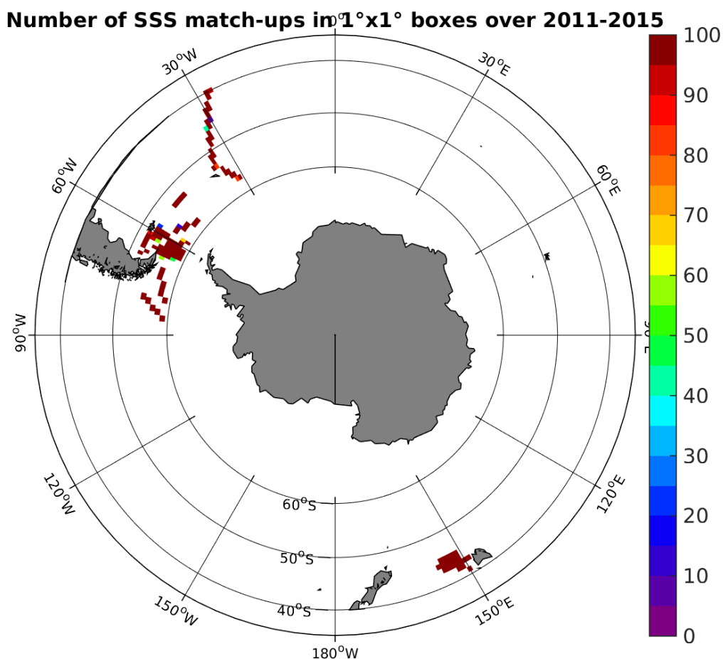
Figure 4: Number of SSS match-ups between TSG-SAMOS SSS and the Aquarius-L3-JPL-V4-7DAY-RUNNING SSS product for the Roaring Forties and Furious Fifties Pi-MEP region over 1^\circ \times 1^\circ boxes and for the full satellite product period.
