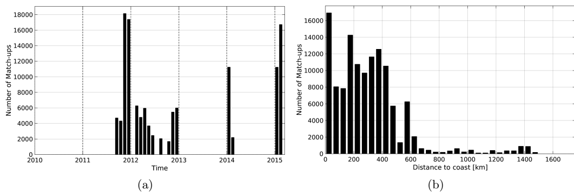
Figure 1: Number of match-ups between TSG-SAMOS and Aquarius-L3-JPL-V4-7DAY-RUNNING SSS as a function of time (a) and as function of the distance to coast (b) over the Roaring Forties and Furious Fifties Pi-MEP region and for the full satellite product period.
