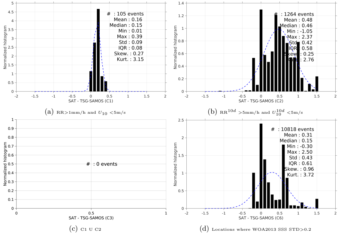
Figure 13: Normalized histogram of \Delta\text{SSS} (Aquarius-L3-JPL-V4-7DAY-RUNNING - TSG-SAMOS) for 6 different subdatasets corresponding to: RR > 1mm/h and U_{10} < 5\text{m/s} (a), RR^{10d} > 5\text{mm/h} and U_{10}^{10d} < 5\text{m/s} (b), C1 U C2 (c), Locations where WOA2013 SSS STD > 0.2 (d).
