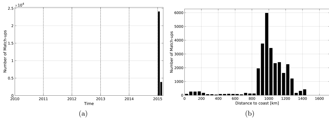
Figure 1: Number of match-ups between TSG-GOSUD-Research-vessel and Aquarius-L3-JPL-V4-7DAY-RUNNING SSS as a function of time (a) and as function of the distance to coast (b) over the Roaring Forties and Furious Fifties Pi-MEP region and for the full satellite product period.
