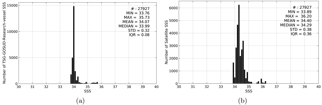
Figure 2: Histograms of SSS from TSG-GOSUD-Research-vessel (a) and Aquarius-L3-JPL-V4-7DAY-RUNNING (b) considering all match-up pairs per bins of 0.1 over the Roaring Forties and Furious Fifties Pi-MEP region and for the full satellite product period.
