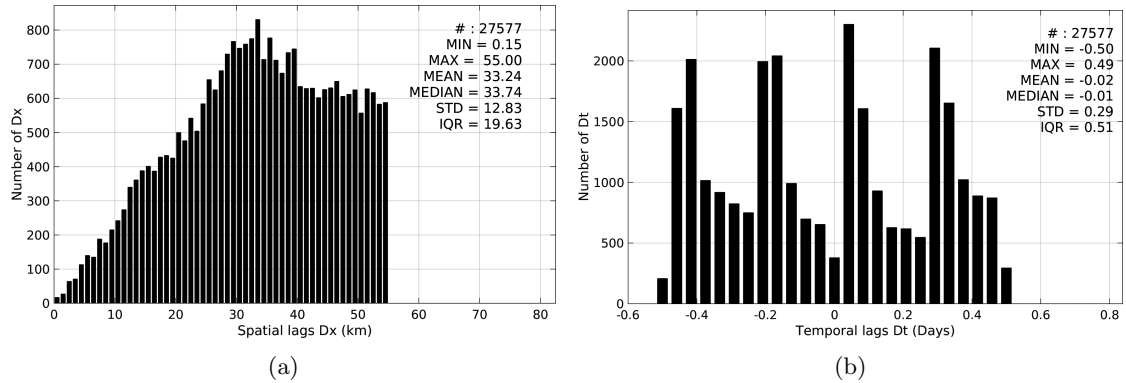
Figure 5: Histograms of the spatial (a) and temporal (b) lags between the time of the Sea mammals measurements and the date of the corresponding Aquarius-L3-JPL-V4-7DAY-RUNNING SSS product.
