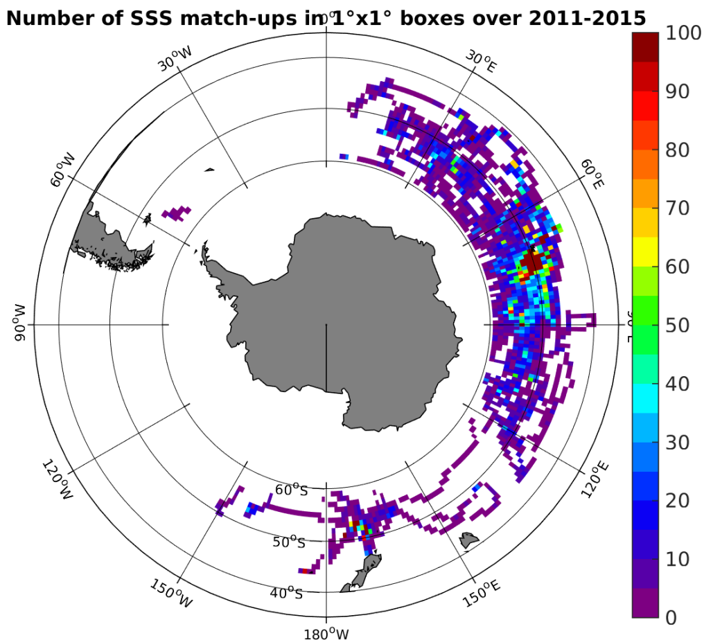
Figure 4: Number of SSS match-ups between Sea mammals SSS and the Aquarius-L3-JPL-V4-7DAY-RUNNING SSS product for the Roaring Forties and Furious Fifties Pi-MEP region over 1^\circ \times 1^\circ boxes and for the full satellite product period.
