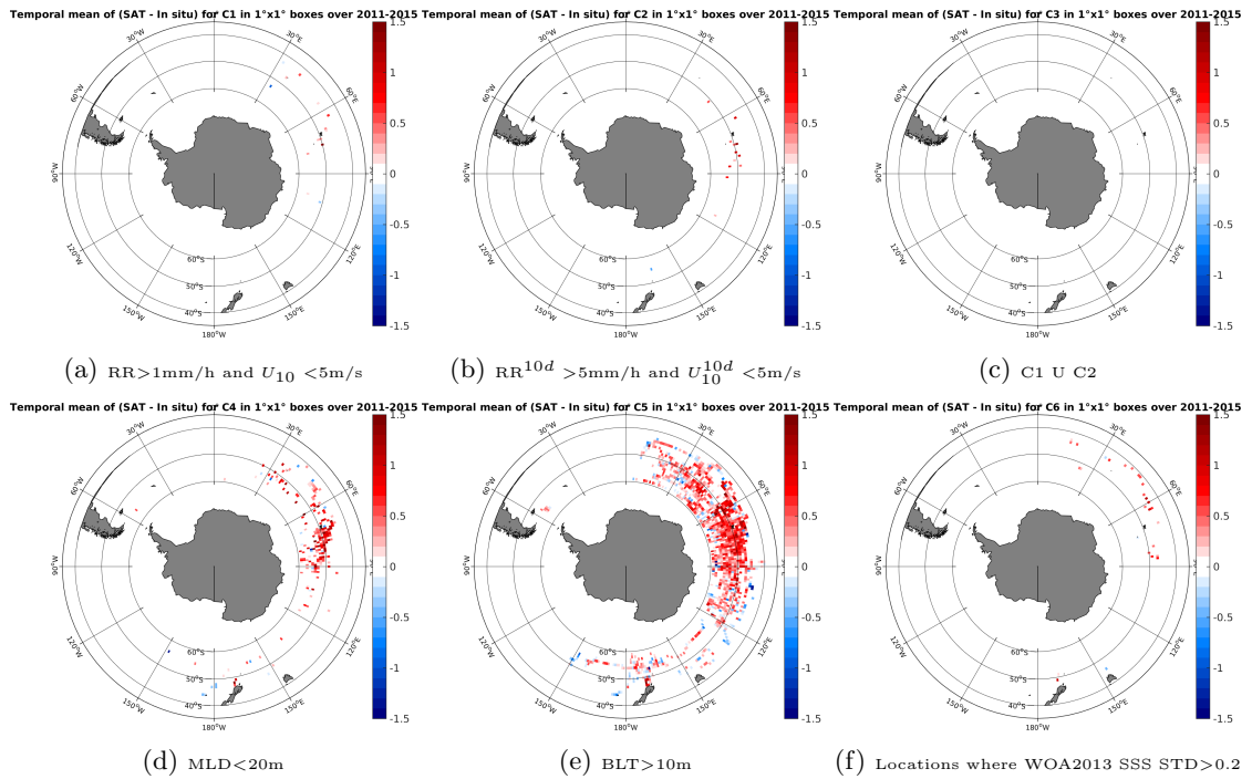
Figure 12: Temporal mean gridded over spatial boxes of size 1^\circ \times 1^\circ of \Delta SSS (Aquarius-L3-JPL-V4-7DAY-RUNNING - Sea mammals) for 6 different subdatasets corresponding to: RR > 1\text{mm/h} and U_{10} < 5\text{m/s} (a), RR^{10d} > 5\text{mm/h} and U_{10}^{10d} < 5\text{m/s} (b), C1 U C2 (c), MLD < 20\text{m} (d), BLT > 10\text{m} (e), Locations where WOA2013 SSS STD > 0.2 (f).
