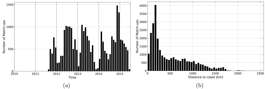
Figure 1: Number of match-ups between Sea mammals and Aquarius-L3-JPL-V4-7DAY-RUNNING SSS as a function of time (a) and as function of the distance to coast (b) over the Roaring Forties and Furious Fifties Pi-MEP region and for the full satellite product period.
