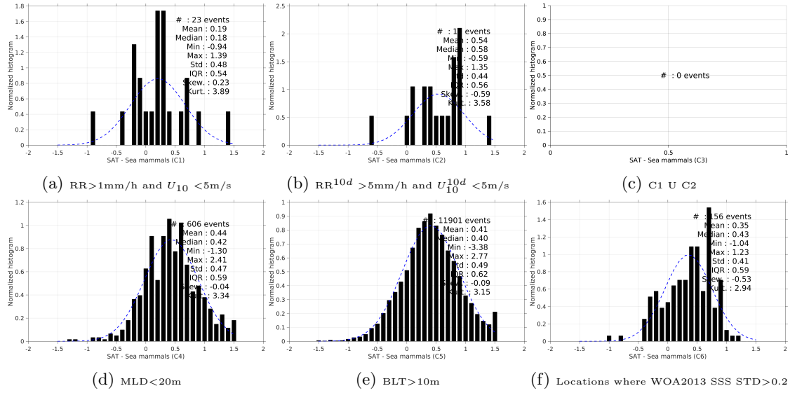
Figure 13: Normalized histogram of \Delta SSS (Aquarius-L3-JPL-V4-7DAY-RUNNING - Sea mammals) for 6 different subdatasets corresponding to: RR > 1mm/h and U_{10} < 5 m/s (a), RR^{10d} > 5 mm/h and U_{10}^{10d} < 5 m/s (b), C1 U C2 (c), MLD < 20m (d), BLT > 10m (e), Locations where WOA2013 SSS STD > 0.2 (f).
