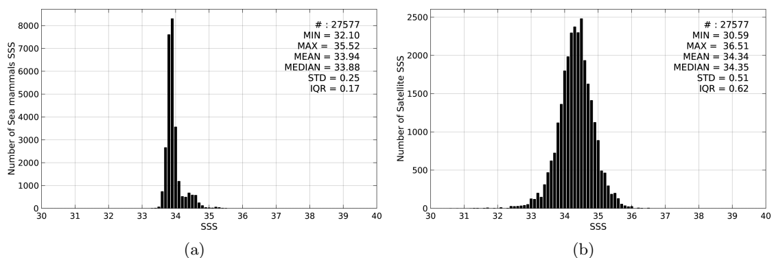
Figure 2: Histograms of SSS from Sea mammals (a) and Aquarius-L3-JPL-V4-7DAY-RUNNING (b) considering all match-up pairs per bins of 0.1 over the Roaring Forties and Furious Fifties Pi-MEP region and for the full satellite product period.
