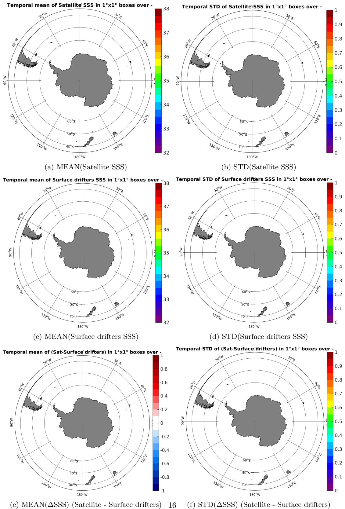
Figure 5: Temporal mean (left) and STD (right) of SSS from Aquarius-L3-JPL-V4-7DAY-RUNNING (top), Surface drifters (middle), and of \Delta SSS (Satellite - Surface drifters). Only match-up pairs are used to generate these maps.
