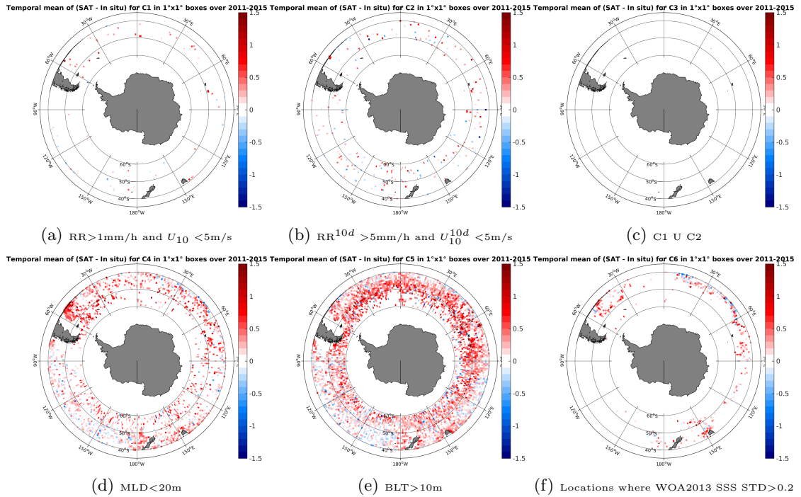
Figure 12: Temporal mean gridded over spatial boxes of size 1^\circ \times 1^\circ of \Delta SSS (Aquarius-L3-JPL-V4-7DAY-RUNNING - Argo) for 6 different subdatasets corresponding to: RR > 1\text{mm/h} and U_{10} < 5\text{m/s} (a), RR^{10d} > 5\text{mm/h} and U_{10}^{10d} < 5\text{m/s} (b), C1 U C2 (c), MLD < 20\text{m} (d), BLT > 10\text{m} (e), Locations where WOA2013 SSS STD > 0.2 (f).
