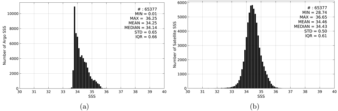
Figure 2: Histograms of SSS from Argo (a) and Aquarius-L3-JPL-V4-7DAY-RUNNING (b) considering all match-up pairs per bins of 0.1 over the Roaring Forties and Furious Fifties Pi-MEP region and for the full satellite product period.
