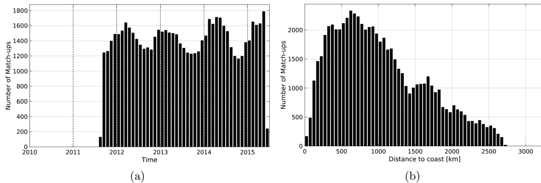
Figure 1: Number of match-ups between Argo and Aquarius-L3-JPL-V4-7DAY-RUNNING SSS as a function of time (a) and as function of the distance to coast (b) over the Roaring Forties and Furious Fifties Pi-MEP region and for the full satellite product period.
