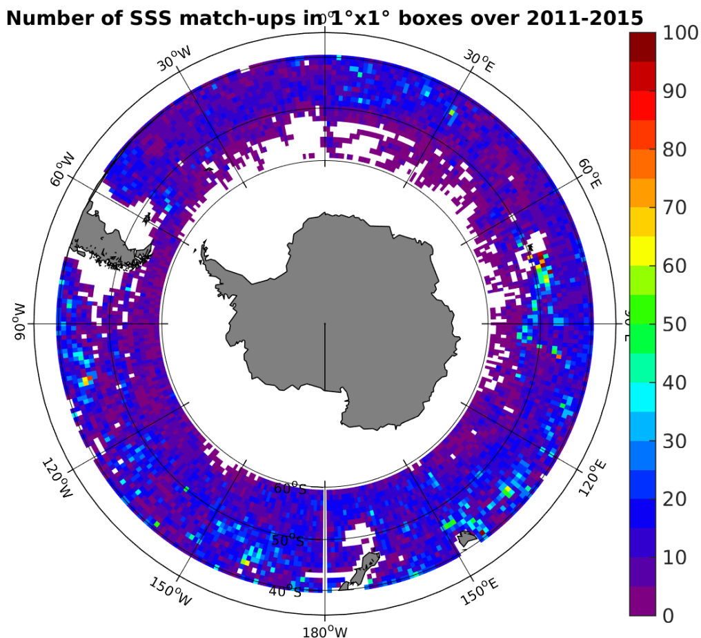
Figure 4: Number of SSS match-ups between Argo SSS and the Aquarius-L3-JPL-V4-7DAY-RUNNING SSS product for the Roaring Forties and Furious Fifties Pi-MEP region over 1^\circ \times 1^\circ boxes and for the full satellite product period.
