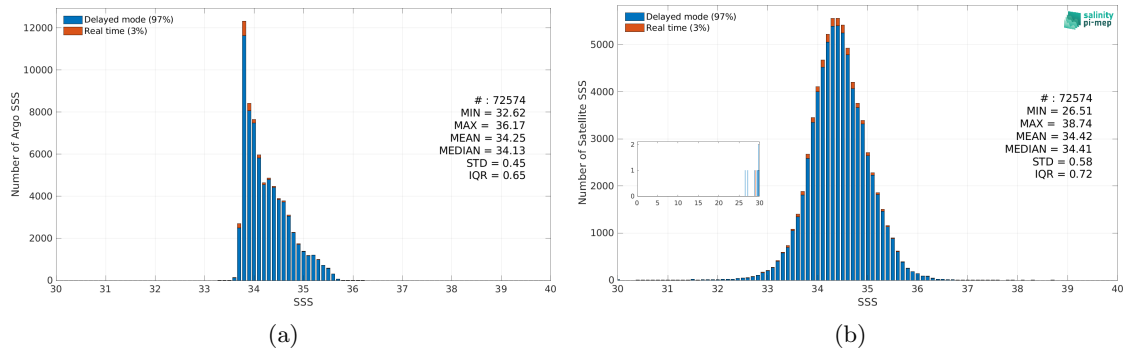
Figure 3: Histograms of SSS from Argo (a) and Aquarius SSS L2-AVERAGED CAP v5 (JPL) (b) considering all match-up pairs per bins of 0.1 over the Roaring Forties and Furious Fifties Pi-MEP region and for the full satellite product period.
