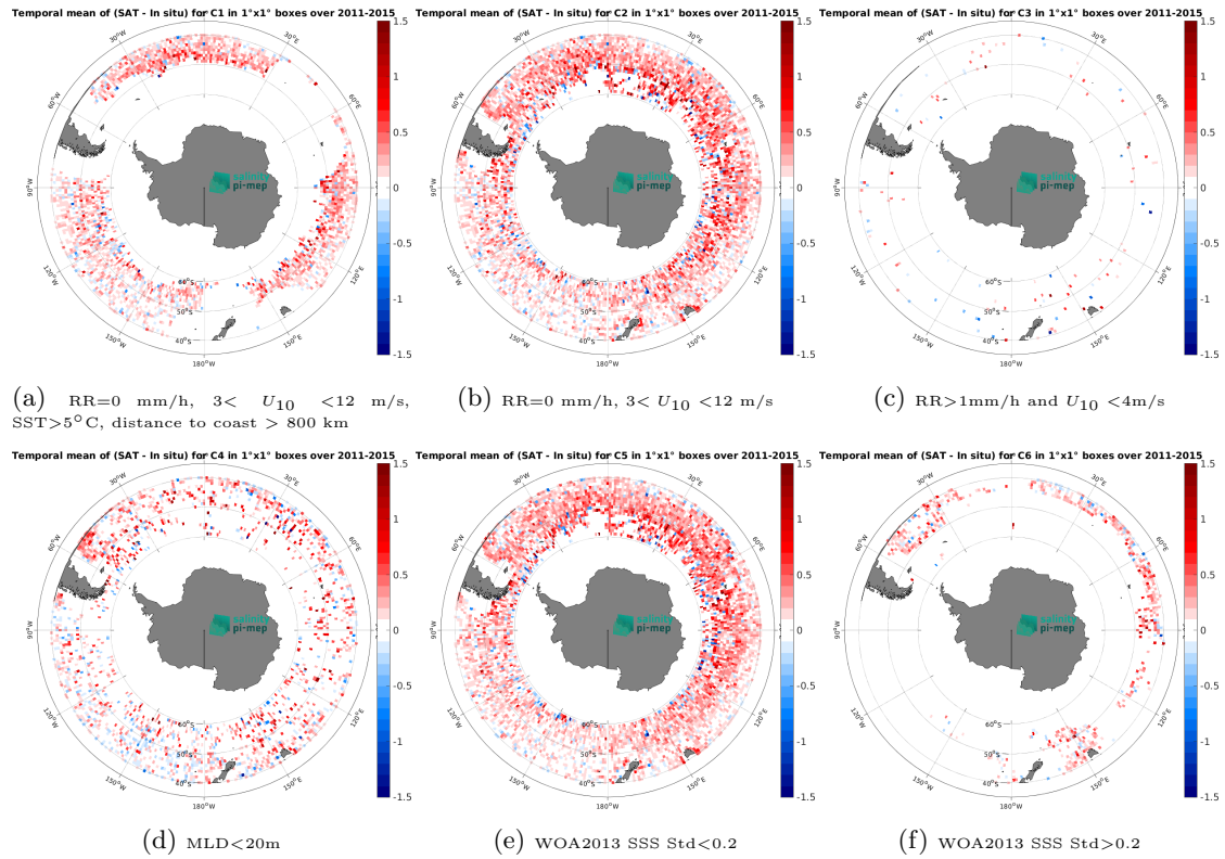
Figure 14: Temporal mean gridded over spatial boxes of size 1^\circ \times 1^\circ of \Delta SSS (Aquarius SSS L2-AVERAGED CAP v5 (JPL) - Argo) for 6 different subdatasets corresponding to:RR=0 mm/h, 3 < U_{10} < 12 m/s, SST >5^\circ C, distance to coast > 800 km (a), RR=0 mm/h, 3 < U_{10} < 12 m/s (b), RR >1 mm/h and U_{10} < 4 m/s (c),MLD <20 m (d),WOA2013 SSS Std <0.2 (e),WOA2013 SSS Std >0.2 (f).
