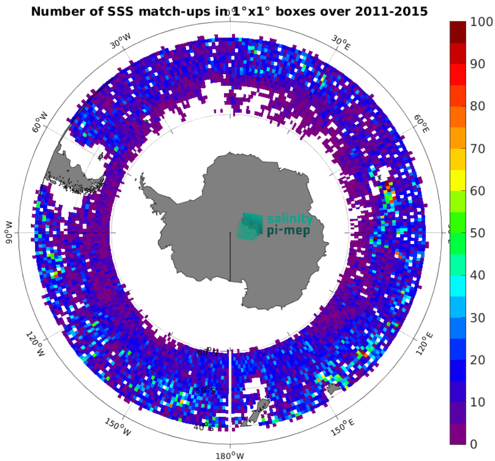
Figure 5: Number of SSS match-ups between Argo SSS and the Aquarius SSS L2-AVERAGED CAP v5 (JPL) SSS product for the Roaring Forties and Furious Fifties Pi-MEP region over 1^\circ \times 1^\circ boxes and for the full satellite product period.
