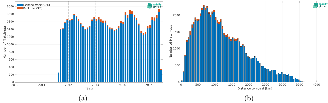
Figure 2: Number of match-ups between Argo and Aquarius SSS L2-AVERAGED CAP v5 (JPL) SSS as a function of time (a) and as function of the distance to coast (b) over the Roaring Forties and Furious Fifties Pi-MEP region and for the full satellite product period.
