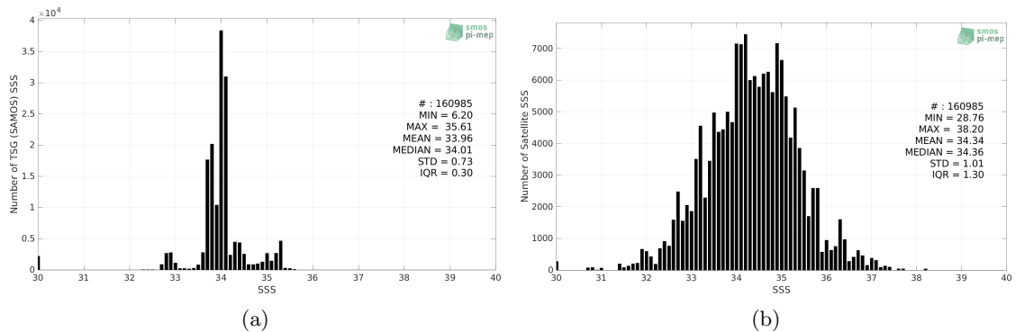
Figure 2: Histograms of SSS from TSG (SAMOS) (a) and Aquarius SSS L2 CAP v5 (JPL) (b) considering all match-up pairs per bins of 0.1 over the Roaring Forties and Furious Fifties Pi-MEP region and for the full satellite product period.
