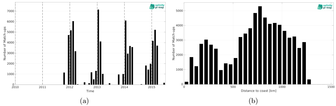
Figure 2: Number of match-ups between TSG (LEGOS-DM) and Aquarius SSS L2 CAP v5 (JPL) SSS as a function of time (a) and as function of the distance to coast (b) over the Roaring Forties and Furious Fifties Pi-MEP region and for the full satellite product period.
