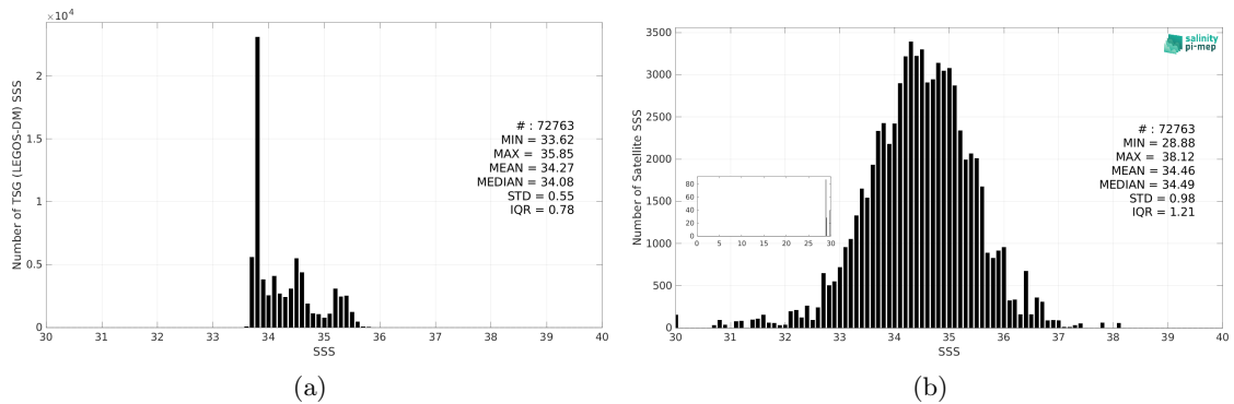
Figure 3: Histograms of SSS from TSG (LEGOS-DM) (a) and Aquarius SSS L2 CAP v5 (JPL) (b) considering all match-up pairs per bins of 0.1 over the Roaring Forties and Furious Fifties Pi-MEP region and for the full satellite product period.
