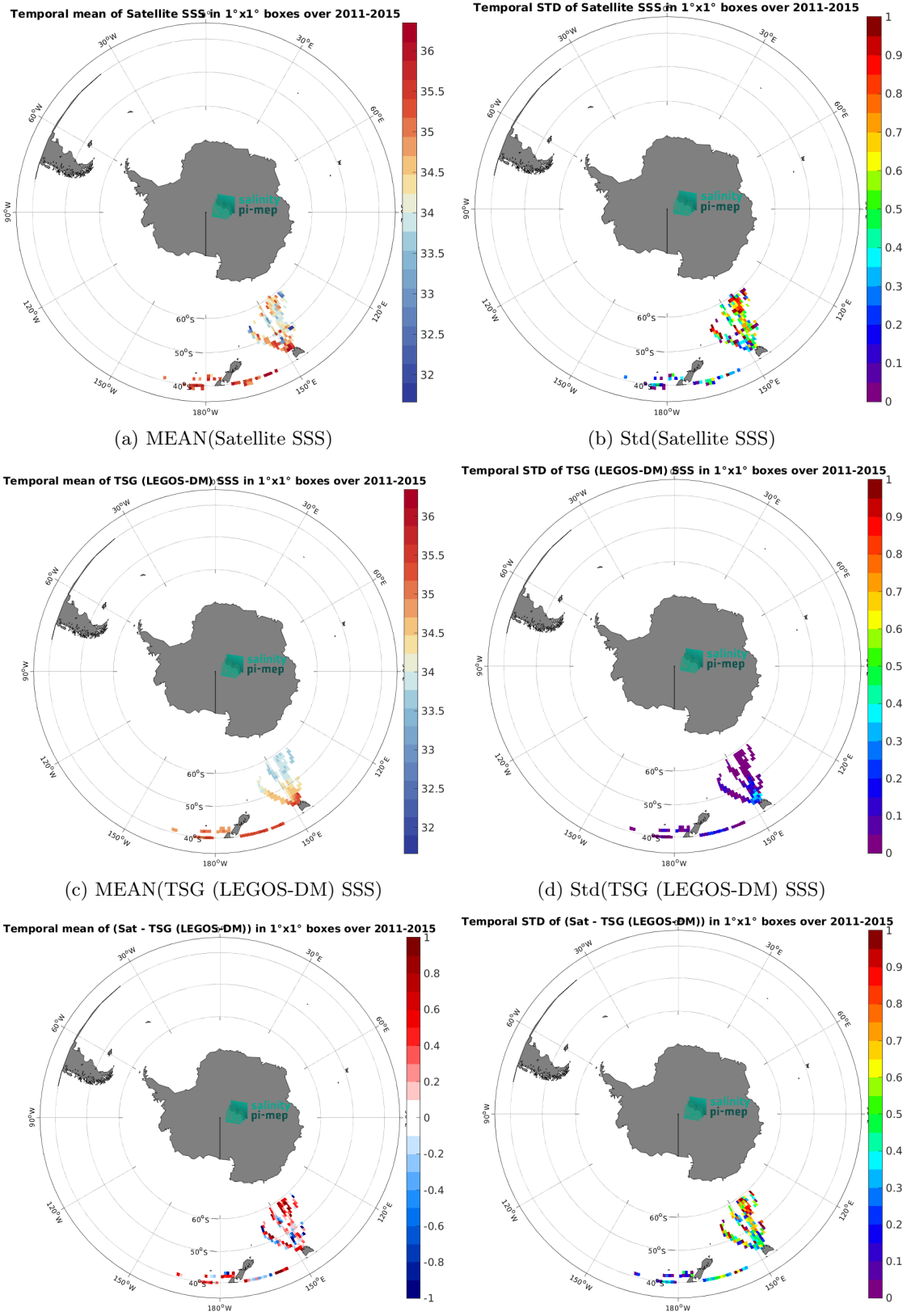
(e) MEAN( \Delta SSS) (Satellite - TSG (LEGOS-DM)) 17 (f) Std( \Delta SSS) (Satellite - TSG (LEGOS-DM)) Figure 7: Temporal mean (left) and Std (right) of SSS from Aquarius SSS L2 CAP v5 (JPL) (top), TSG (LEGOS-DM) (middle), and of \Delta SSS (Satellite - TSG (LEGOS-DM)). Only match-up pairs are used to generate these maps.
