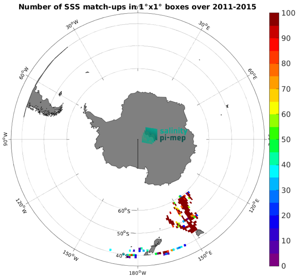
Figure 5: Number of SSS match-ups between TSG (LEGOS-DM) SSS and the Aquarius SSS L2 CAP v5 (JPL) SSS product for the Roaring Forties and Furious Fifties Pi-MEP region over 1^\circ \times 1^\circ boxes and for the full satellite product period.
