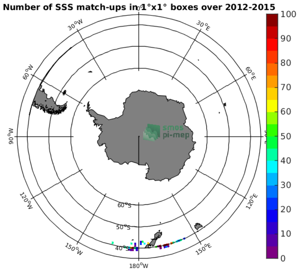
Figure 4: Number of SSS match-ups between TSG-LEGOS-DM SSS and the Aquarius-L2-JPL-V5 SSS product for the Roaring Forties and Furious Fifties Pi-MEP region over 1^\circ \times 1^\circ boxes and for the full satellite product period.
