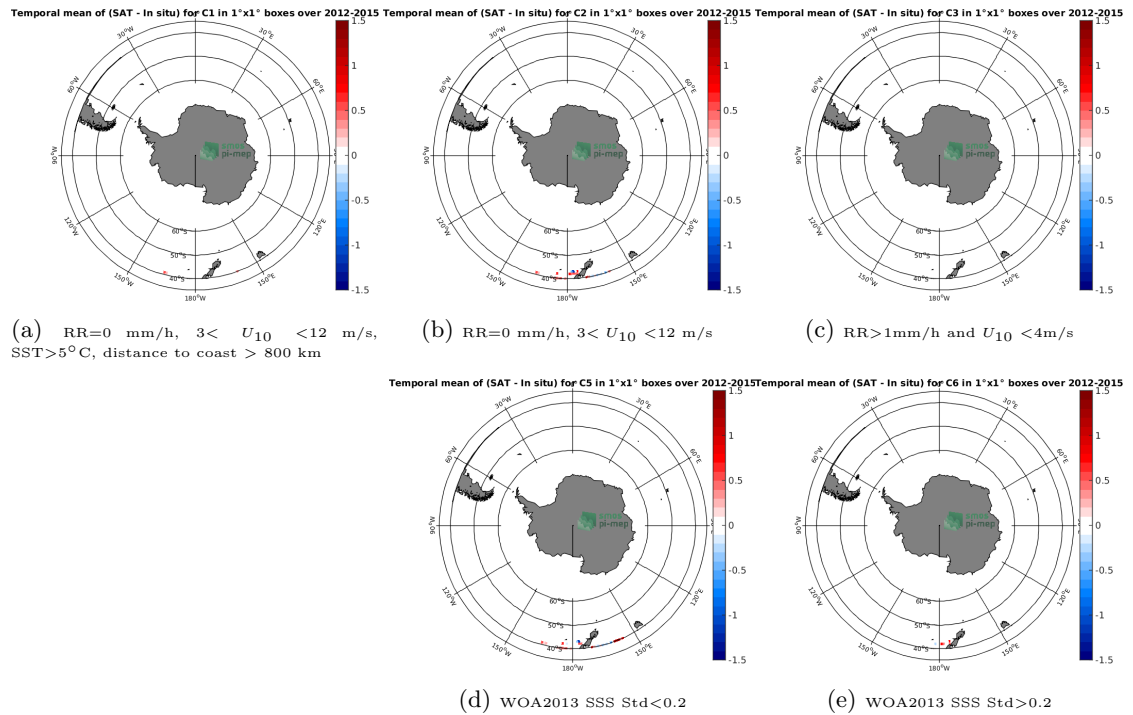
Figure 12: Temporal mean gridded over spatial boxes of size 1^\circ \times 1^\circ of \Delta SSS (Aquarius-L2-JPL-V5 - TSG-LEGOS-DM) for 5 different subdatasets corresponding to:RR=0 mm/h, 3 < U_{10} < 12 m/s, SST >5^\circ C, distance to coast > 800 km (a), RR=0 mm/h, 3 < U_{10} < 12 m/s (b), RR >1 mm/h and U_{10} < 4 m/s (c), WOA2013 SSS Std <0.2 (d), WOA2013 SSS Std >0.2 (e).
