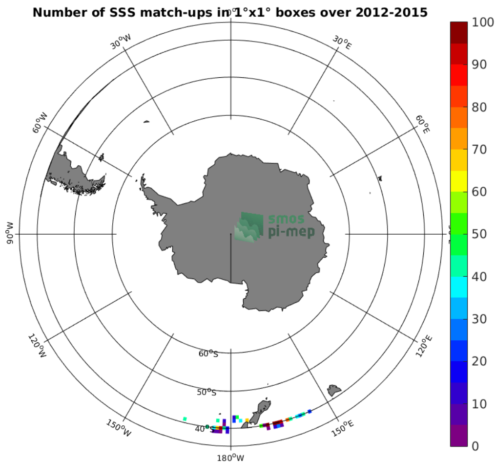
Figure 4: Number of SSS match-ups between TSG-LEGOS-DM SSS and the Aquarius-L2-JPL-V5 SSS product for the Roaring Forties and Furious Fifties Pi-MEP region over 1^\circ \times 1^\circ boxes and for the full satellite product period.
