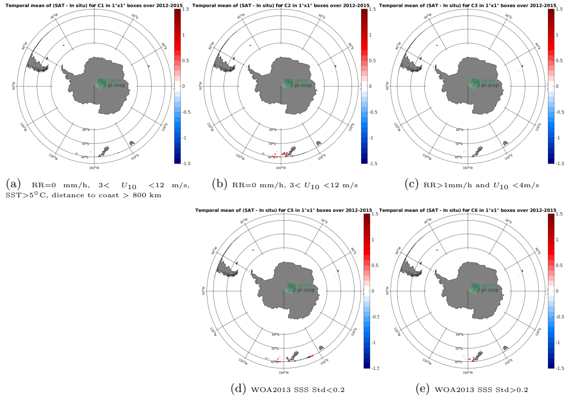
Figure 12: Temporal mean gridded over spatial boxes of size 1^\circ \times 1^\circ of \Delta SSS (Aquarius-L2-JPL-V5 - TSG-LEGOS-DM) for 5 different subdatasets corresponding to:RR=0 mm/h, 3 < U_{10} < 12 m/s, SST >5^\circ C, distance to coast > 800 km (a), RR=0 mm/h, 3 < U_{10} < 12 m/s (b), RR >1 mm/h and U_{10} < 4 m/s (c), WOA2013 SSS Std <0.2 (d), WOA2013 SSS Std >0.2 (e).
