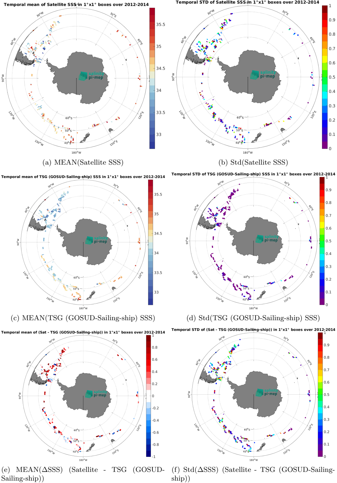
Figure 7: Temporal mean (left) and Std (right) of SSS from Aquarius SSS L2 CAP v5 (JPL) (top), TSG (GOSUD-Sailing-ship) (middle), and of \Delta SSS (Satellite - TSG (GOSUD-Sailing-ship)). Only match-up pairs are used to generate these maps.
