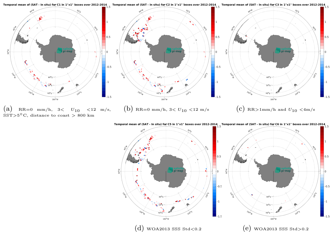
Figure 14: Temporal mean gridded over spatial boxes of size 1^\circ \times 1^\circ of \Delta SSS (Aquarius SSS L2 CAP v5 (JPL) - TSG (GOSUD-Sailing-ship)) for 5 different subdatasets corresponding to: RR=0 mm/h, 3 < U_{10} < 12 m/s, SST > 5^\circ\text{C} , distance to coast > 800 km (a), RR=0 mm/h, 3 < U_{10} < 12 m/s (b), RR > 1 mm/h and U_{10} < 4 m/s (c), WOA2013 SSS Std < 0.2 (d), WOA2013 SSS Std > 0.2 (e).
