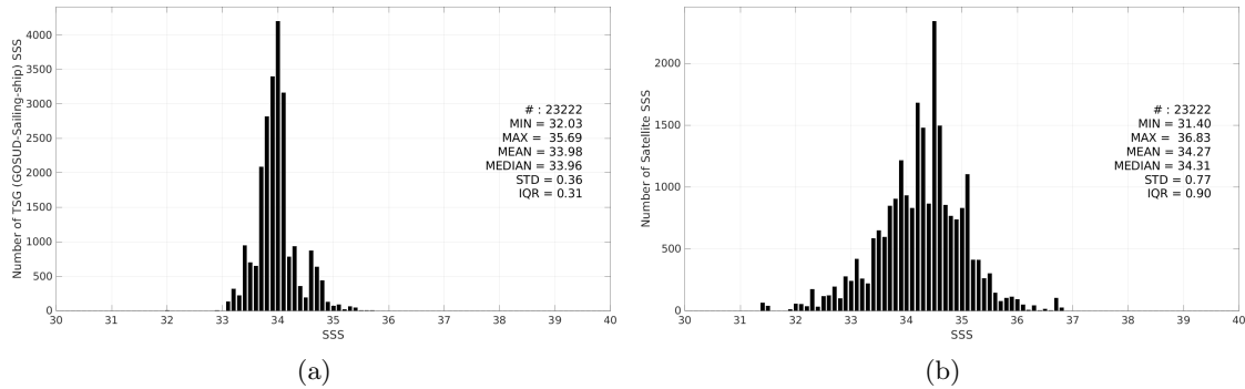
Figure 3: Histograms of SSS from TSG (GOSUD-Sailing-ship) (a) and Aquarius SSS L2 CAP v5 (JPL) (b) considering all match-up pairs per bins of 0.1 over the Roaring Forties and Furious Fifties Pi-MEP region and for the full satellite product period.
