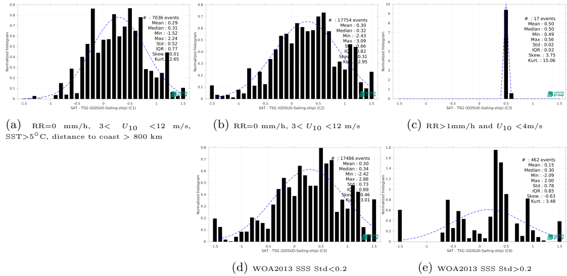
Figure 15: Normalized histogram of \Delta\text{SSS} (Aquarius SSS L2 CAP v5 (JPL) - TSG (GOSUD-Sailing-ship)) for 5 different subdatasets corresponding to: RR=0 mm/h, 3 < U_{10} < 12 m/s, SST > 5^\circ\text{C} , distance to coast > 800 km (a), RR=0 mm/h, 3 < U_{10} < 12 m/s (b), RR > 1 mm/h and U_{10} < 4 m/s (c), WOA2013 SSS Std < 0.2 (d), WOA2013 SSS Std > 0.2 (e).
