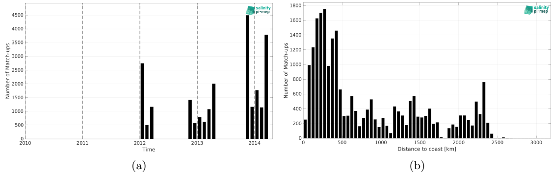
Figure 2: Number of match-ups between TSG (GOSUD-Sailing-ship) and Aquarius SSS L2 CAP v5 (JPL) SSS as a function of time (a) and as function of the distance to coast (b) over the Roaring Forties and Furious Fifties Pi-MEP region and for the full satellite product period.
