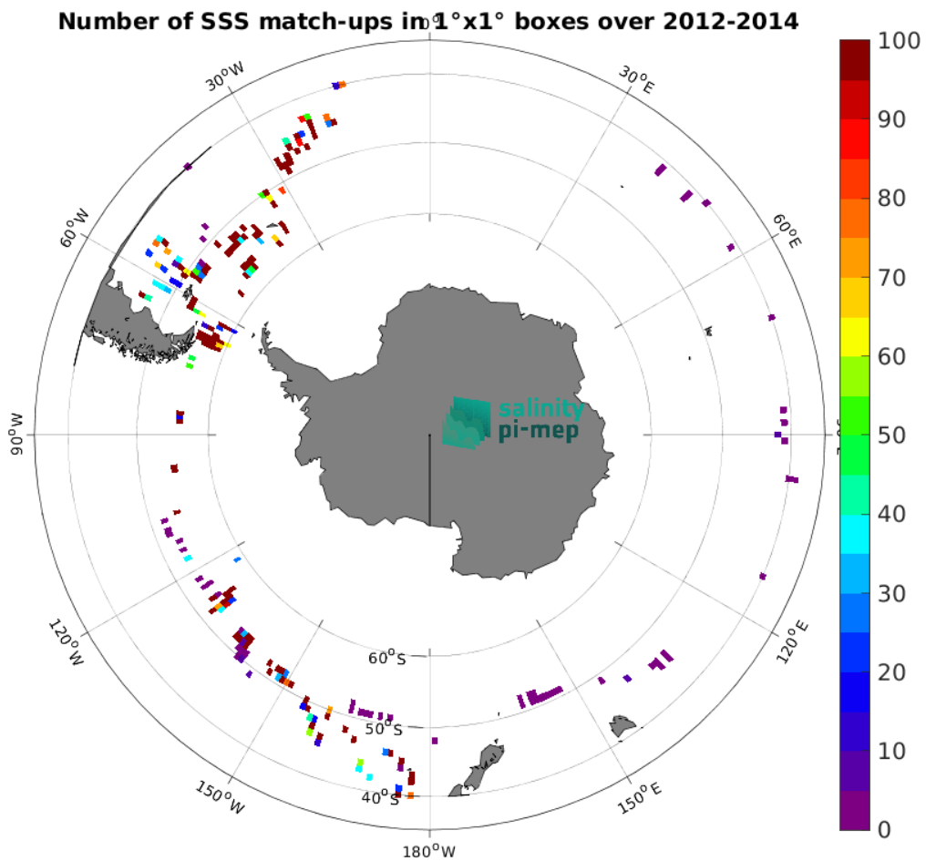
Figure 5: Number of SSS match-ups between TSG (GOSUD-Sailing-ship) SSS and the Aquarius SSS L2 CAP v5 (JPL) SSS product for the Roaring Forties and Furious Fifties Pi-MEP region over 1^\circ \times 1^\circ boxes and for the full satellite product period.
