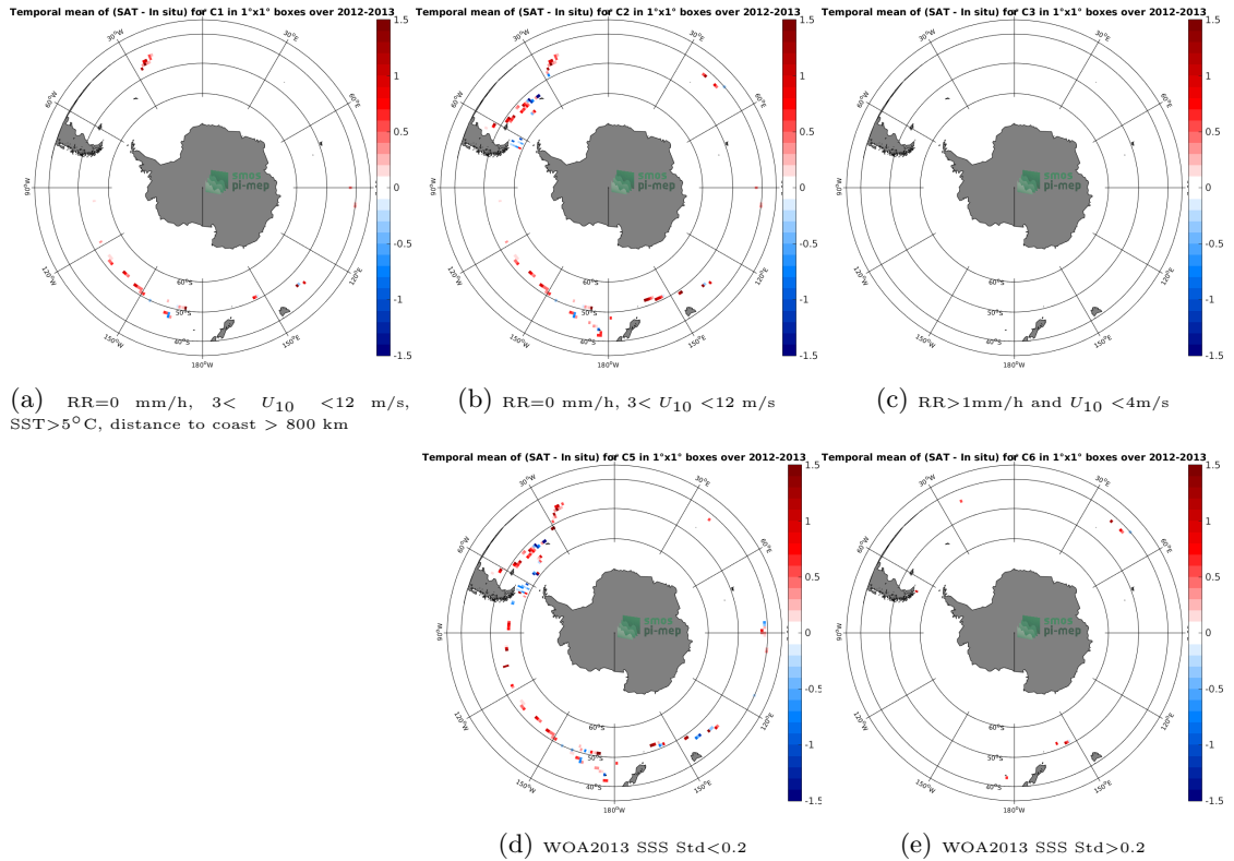
Figure 12: Temporal mean gridded over spatial boxes of size 1^\circ \times 1^\circ of \Delta SSS (Aquarius-L2-JPL-V5 - TSG-GOSUD-Sailing-ship) for 5 different subdatasets corresponding to:RR=0 mm/h, 3 < U_{10} < 12 m/s, SST > 5^\circ\text{C} , distance to coast > 800 km (a), RR=0 mm/h, 3 < U_{10} < 12 m/s (b), RR > 1 mm/h and U_{10} < 4 m/s (c), WOA2013 SSS Std < 0.2 (d), WOA2013 SSS Std > 0.2 (e).
