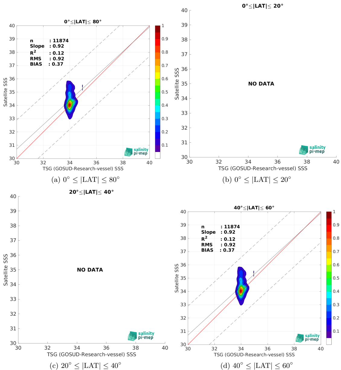
Figure 10: Contour maps of the concentration of Aquarius SSS L2 CAP v5 (JPL) SSS (y-axis) versus TSG (GOSUD-Research-vessel) SSS (x-axis) at match-up pairs for different latitude bands. For each plot, the red line shows x=y . The black thin and dashed lines indicate a linear fit through the data cloud and the \pm 95\% confidence levels, respectively. The number match-up pairs n , the slope and R^2 coefficient of the linear fit, the root mean square (RMS) and the mean bias between satellite and in situ data are indicated for each latitude band in each plots.
