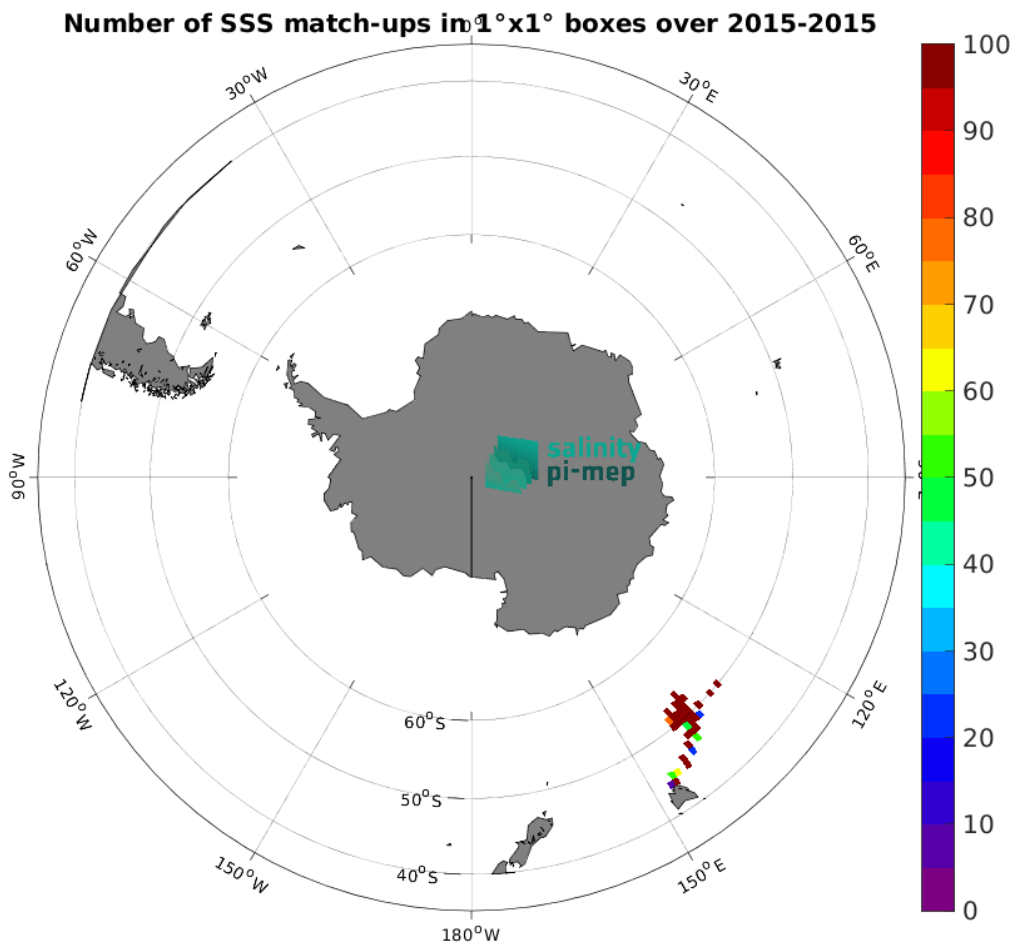
Figure 5: Number of SSS match-ups between TSG (GOSUD-Research-vessel) SSS and the Aquarius SSS L2 CAP v5 (JPL) SSS product for the Roaring Forties and Furious Fifties Pi-MEP region over 1^\circ \times 1^\circ boxes and for the full satellite product period.
