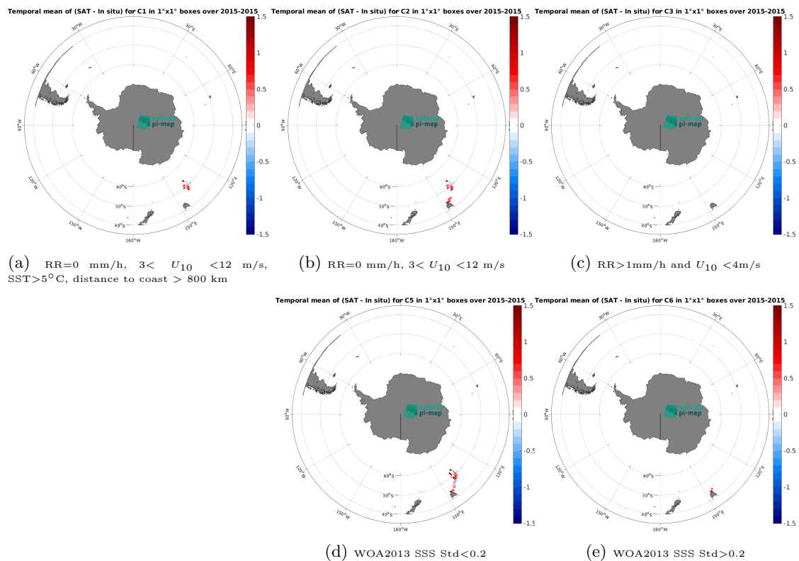
Figure 14: Temporal mean gridded over spatial boxes of size 1^\circ \times 1^\circ of \Delta SSS (Aquarius SSS L2 CAP v5 (JPL) - TSG (GOSUD-Research-vessel)) for 5 different subdatasets corresponding to:RR=0 mm/h, 3 < U_{10} < 12 m/s, SST > 5^\circ\text{C} , distance to coast > 800 km (a), RR=0 mm/h, 3 < U_{10} < 12 m/s (b), RR > 1 mm/h and U_{10} < 4 m/s (c), WOA2013 SSS Std < 0.2 (d), WOA2013 SSS Std > 0.2 (e).
