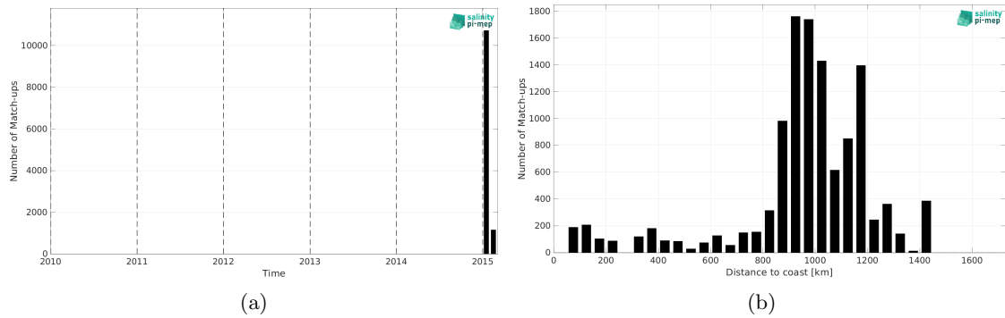
Figure 2: Number of match-ups between TSG (GOSUD-Research-vessel) and Aquarius SSS L2 CAP v5 (JPL) SSS as a function of time (a) and as function of the distance to coast (b) over the Roaring Forties and Furious Fifties Pi-MEP region and for the full satellite product period.
