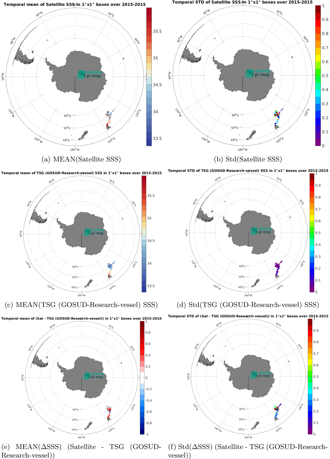
Figure 7: Temporal mean (left) and Std (right) of SSS from Aquarius SSS L2 CAP v5 (JPL) (top), TSG (GOSUD-Research-vessel) (middle), and of \Delta SSS (Satellite - TSG (GOSUD-Research-vessel)). Only match-up pairs are used to generate these maps.
