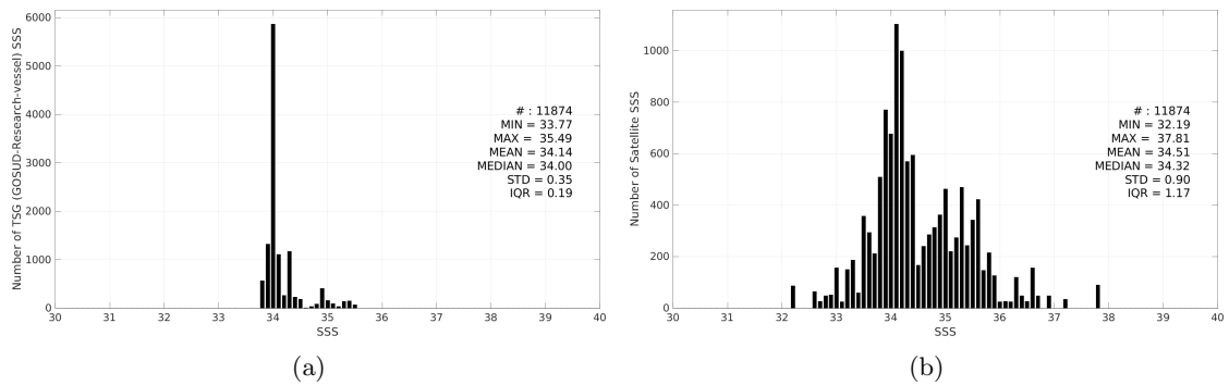
Figure 3: Histograms of SSS from TSG (GOSUD-Research-vessel) (a) and Aquarius SSS L2 CAP v5 (JPL) (b) considering all match-up pairs per bins of 0.1 over the Roaring Forties and Furious Fifties Pi-MEP region and for the full satellite product period.
