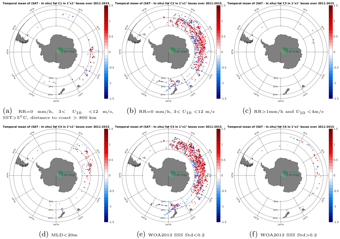
Figure 12: Temporal mean gridded over spatial boxes of size 1^\circ \times 1^\circ of \Delta SSS (Aquarius-L2-JPL-V5 - Sea mammals) for 6 different subdatasets corresponding to:RR=0 mm/h, 3 < U_{10} < 12 m/s, SST >5^\circ C, distance to coast > 800 km (a), RR=0 mm/h, 3 < U_{10} < 12 m/s (b), RR >1 mm/h and U_{10} < 4 m/s (c),MLD <20 m (d),WOA2013 SSS Std <0.2 (e),WOA2013 SSS Std >0.2 (f).
