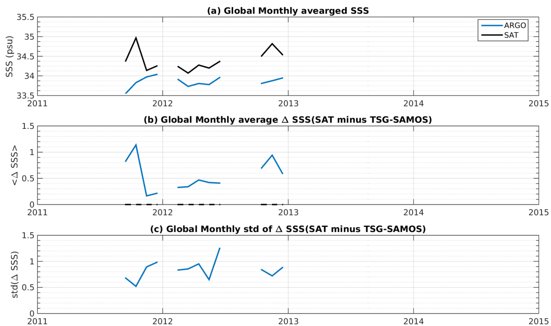
Figure 7: Time series of the monthly averaged mean SSS (top), mean \Delta SSS (Satellite - TSG-SAMOS) and STD of \Delta SSS (Satellite - TSG-SAMOS) over the Roaring Forties and Furious Fifties Pi-MEP region considering all match-ups collected by the Pi-MEP platform.
