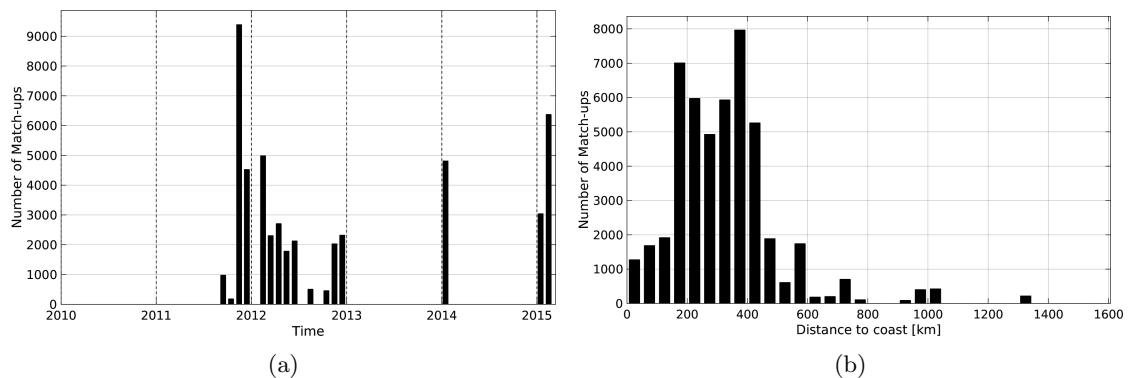
Figure 1: Number of match-ups between TSG-SAMOS and AQUARIUS-L2-JPL-V4 SSS as a function of time (a) and as function of the distance to coast (b) over the Roaring Forties and Furious Fifties Pi-MEP region and for the full satellite product period.
