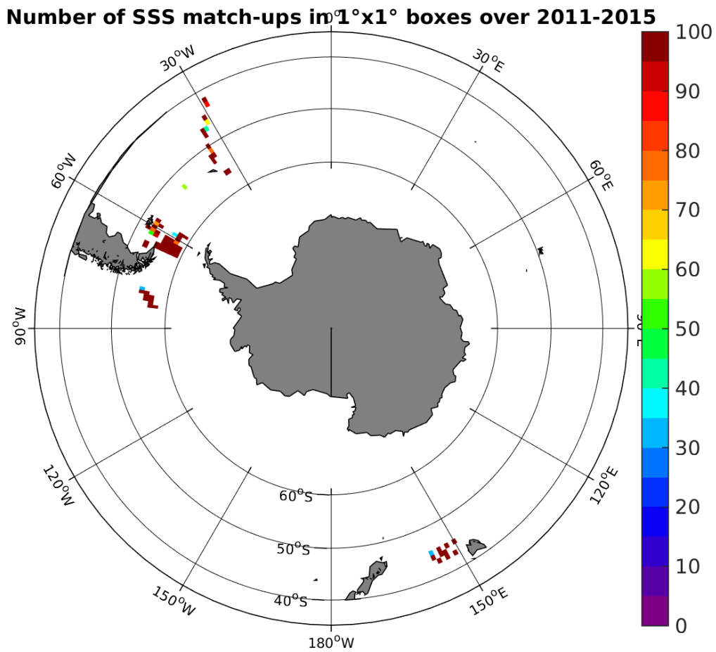
Figure 4: Number of SSS match-ups between TSG-SAMOS SSS and the AQUARIUS-L2-JPL-V4 SSS product for the Roaring Forties and Furious Fifties Pi-MEP region over 1°x1° boxes and for the full satellite product period.
