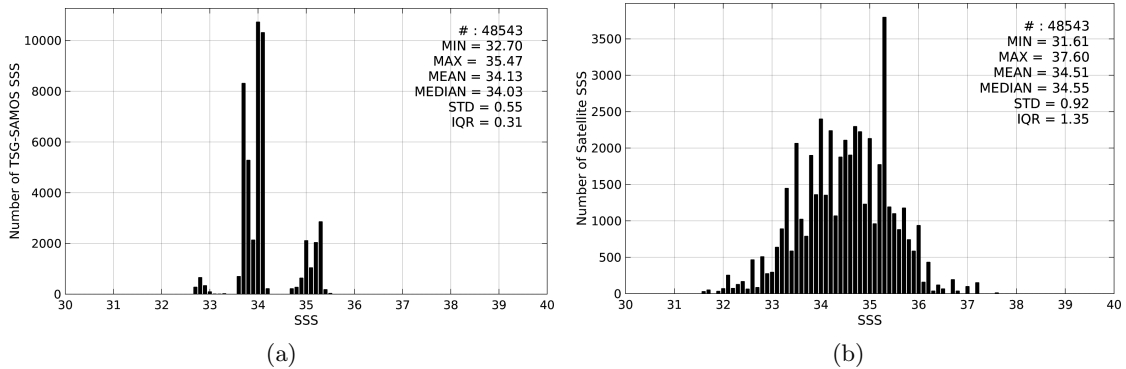
Figure 2: Histograms of SSS from TSG-SAMOS (a) and AQUARIUS-L2-JPL-V4 (b) considering all match-up pairs per bins of 0.1 over the Roaring Forties and Furious Fifties Pi-MEP region and for the full satellite product period.
