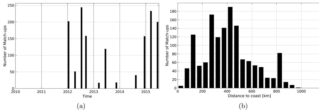
Figure 1: Number of match-ups between TSG-LEGOS-DM and AQUARIUS-L2-JPL-V4 SSS as a function of time (a) and as function of the distance to coast (b) over the Roaring Forties and Furious Fifties Pi-MEP region and for the full satellite product period.
