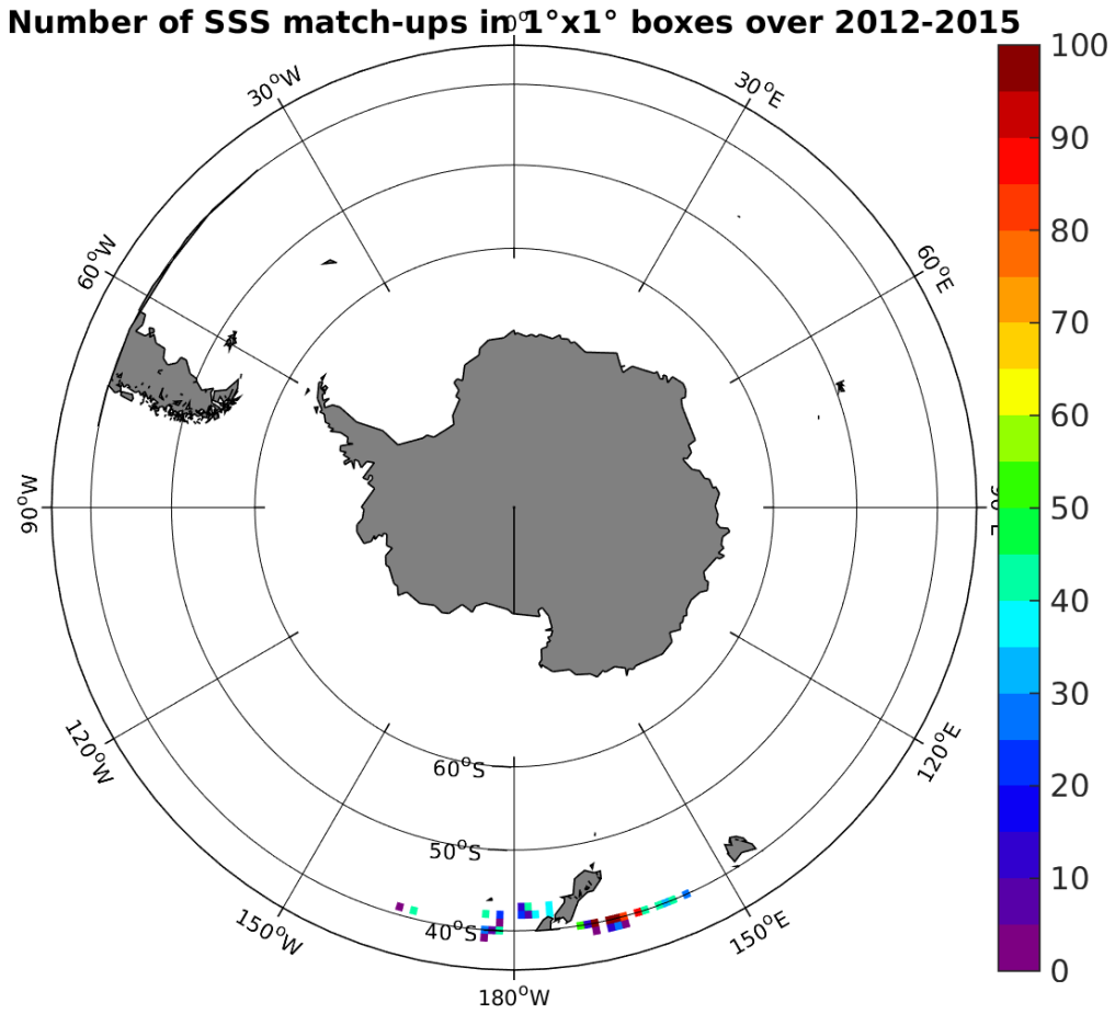
Figure 4: Number of SSS match-ups between TSG-LEGOS-DM SSS and the AQUARIUS-L2-JPL-V4 SSS product for the Roaring Forties and Furious Fifties Pi-MEP region over 1°x1° boxes and for the full satellite product period.
