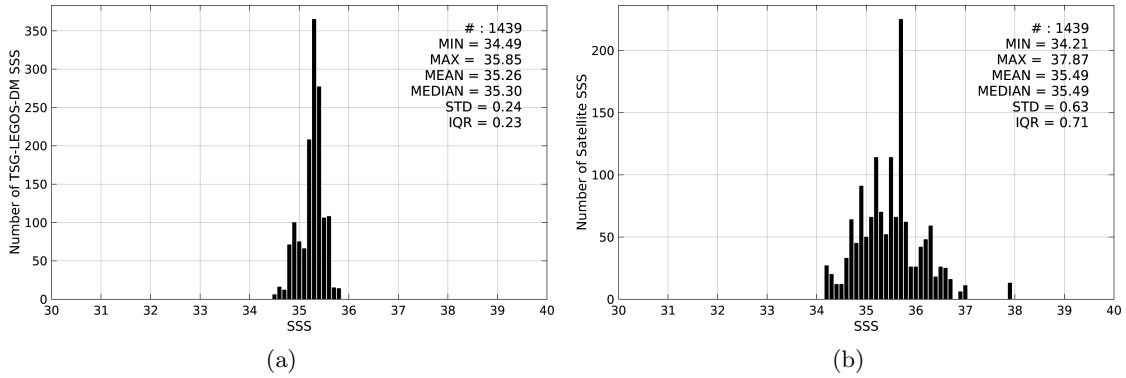
Figure 2: Histograms of SSS from TSG-LEGOS-DM (a) and AQUARIUS-L2-JPL-V4 (b) considering all match-up pairs per bins of 0.1 over the Roaring Forties and Furious Fifties Pi-MEP region and for the full satellite product period.
